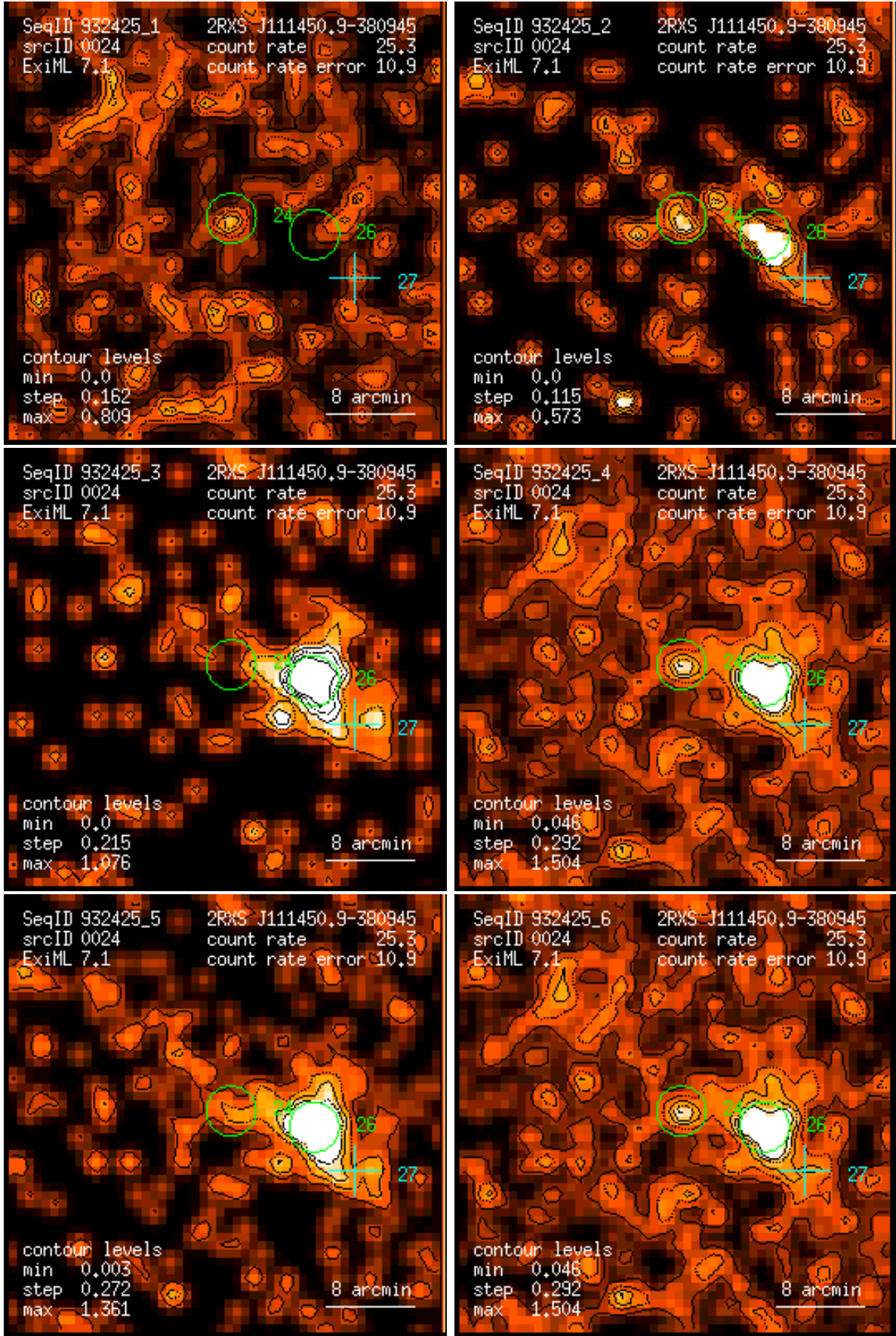
Figure 24: RASS 932425: detection 0024: band rate images, Gaussian filter: (1) PSPC channels 11 – 41, (2) 52 – 90, (3) 91 – 201, (4) 11 – 235, (5) 52 – 201, (6) 11 – 201. Broad band rates in counts/ks. Band rate contour levels in counts/ks/arcmin 2 .
