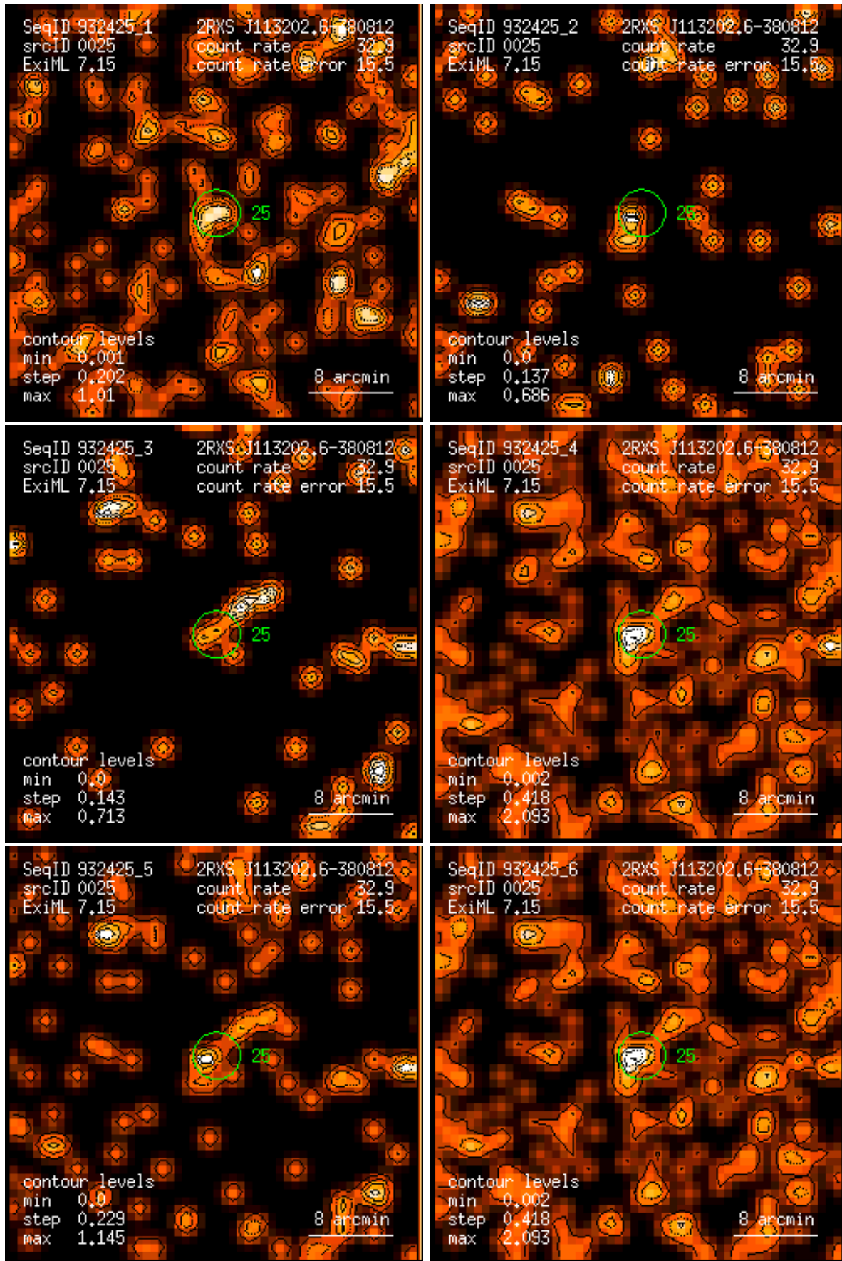
Figure 25: RASS 932425: detection 0025: band rate images, Gaussian filter: (1) PSPC channels 11 – 41, (2) 52 – 90, (3) 91 – 201, (4) 11 – 235, (5) 52 – 201, (6) 11 – 201. Broad band rates in counts/ks. Band rate contour levels in counts/ks/arcmin 2 .
