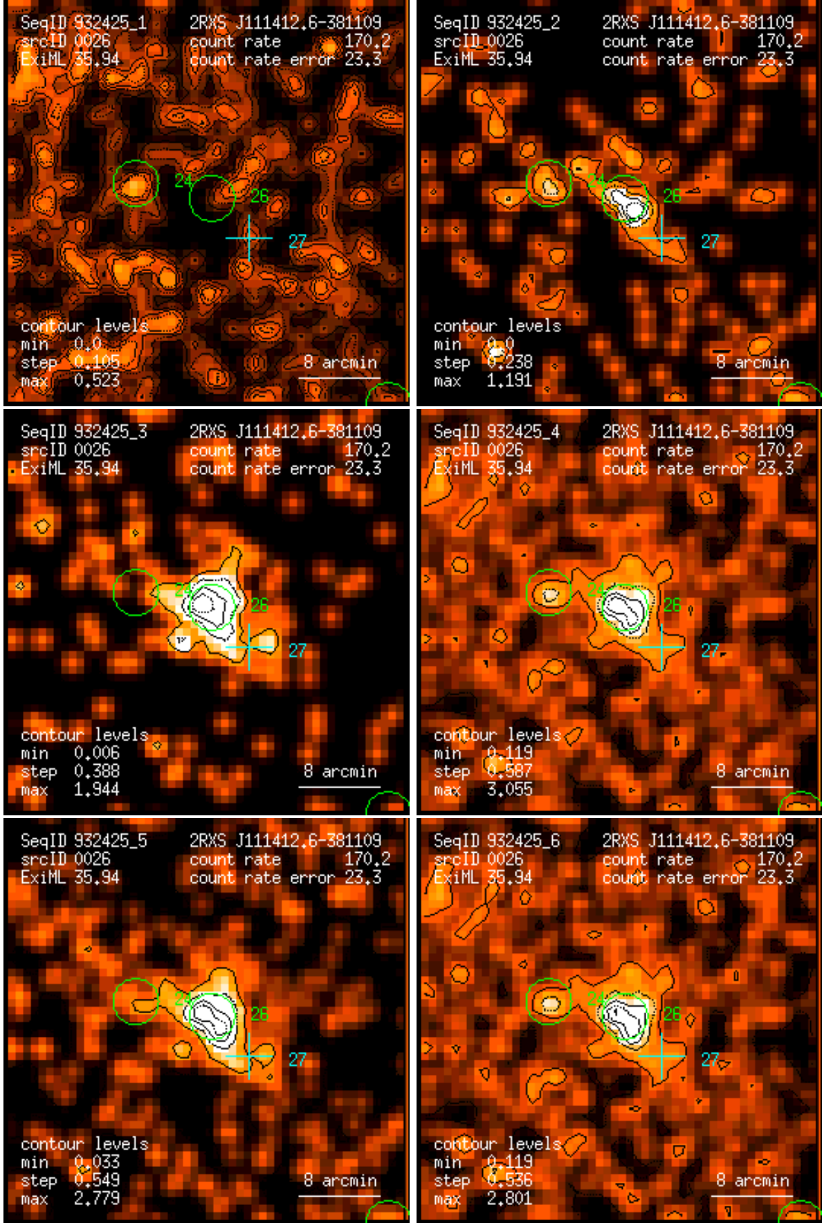
Figure 26: RASS 932425: detection 0026: band rate images, Gaussian filter: (1) PSPC channels 11 – 41, (2) 52 – 90, (3) 91 – 201, (4) 11 – 235, (5) 52 – 201, (6) 11 – 201. Broad band rates in counts/ks. Band rate contour levels in counts/ks/arcmin 2 .
