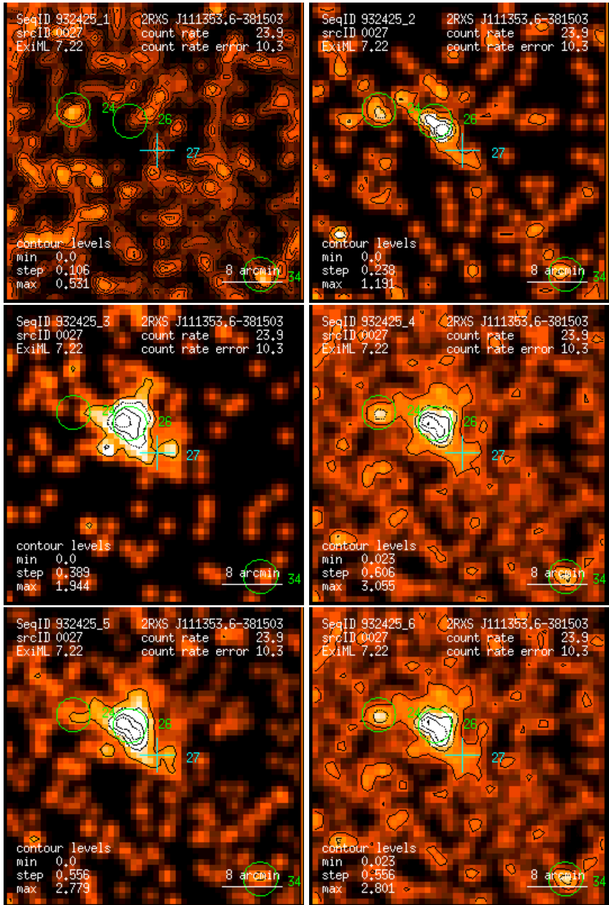
Figure 27: RASS 932425: detection 0027: band rate images, Gaussian filter: (1) PSPC channels 11 – 41, (2) 52 – 90, (3) 91 – 201, (4) 11 – 235, (5) 52 – 201, (6) 11 – 201. Broad band rates in counts/ks. Band rate contour levels in counts/ks/arcmin 2 .
