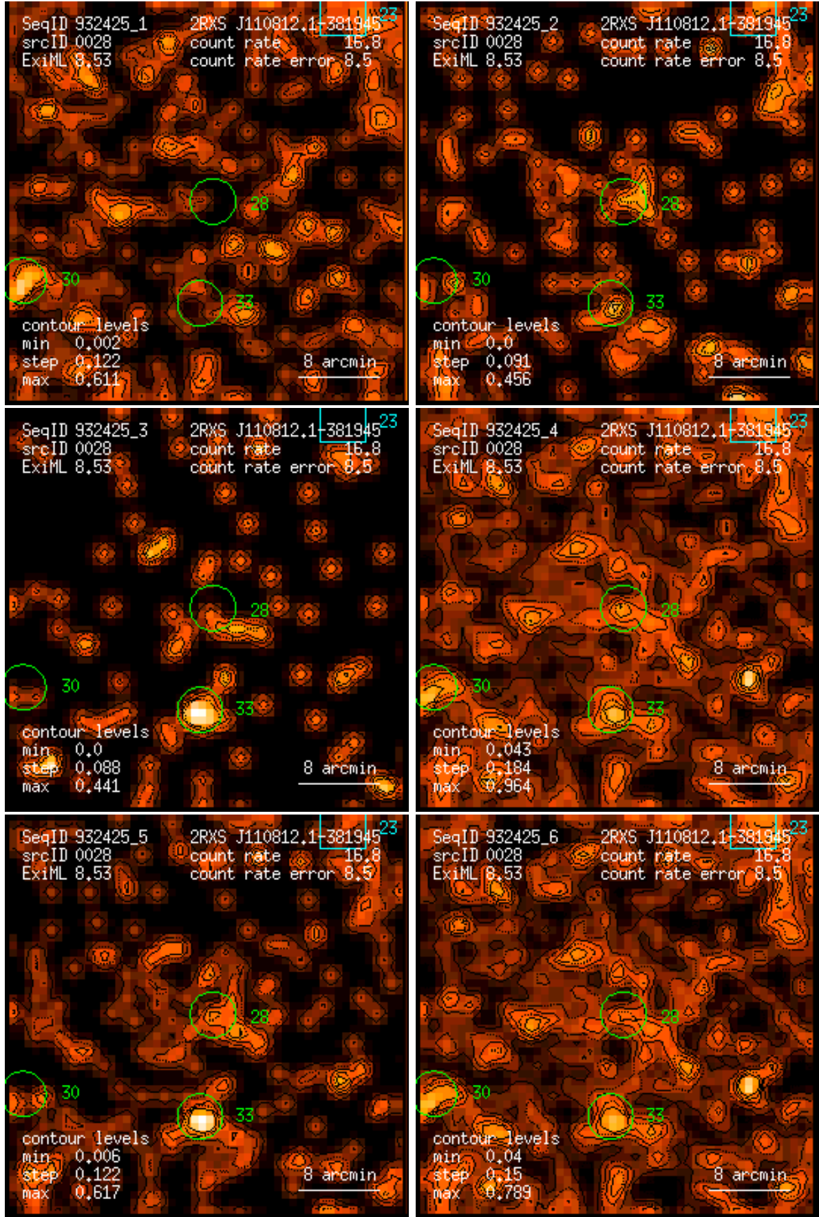
Figure 28: RASS 932425: detection 0028: band rate images, Gaussian filter: (1) PSPC channels 11 – 41, (2) 52 – 90, (3) 91 – 201, (4) 11 – 235, (5) 52 – 201, (6) 11 – 201. Broad band rates in counts/ks. Band rate contour levels in counts/ks/arcmin 2 .
