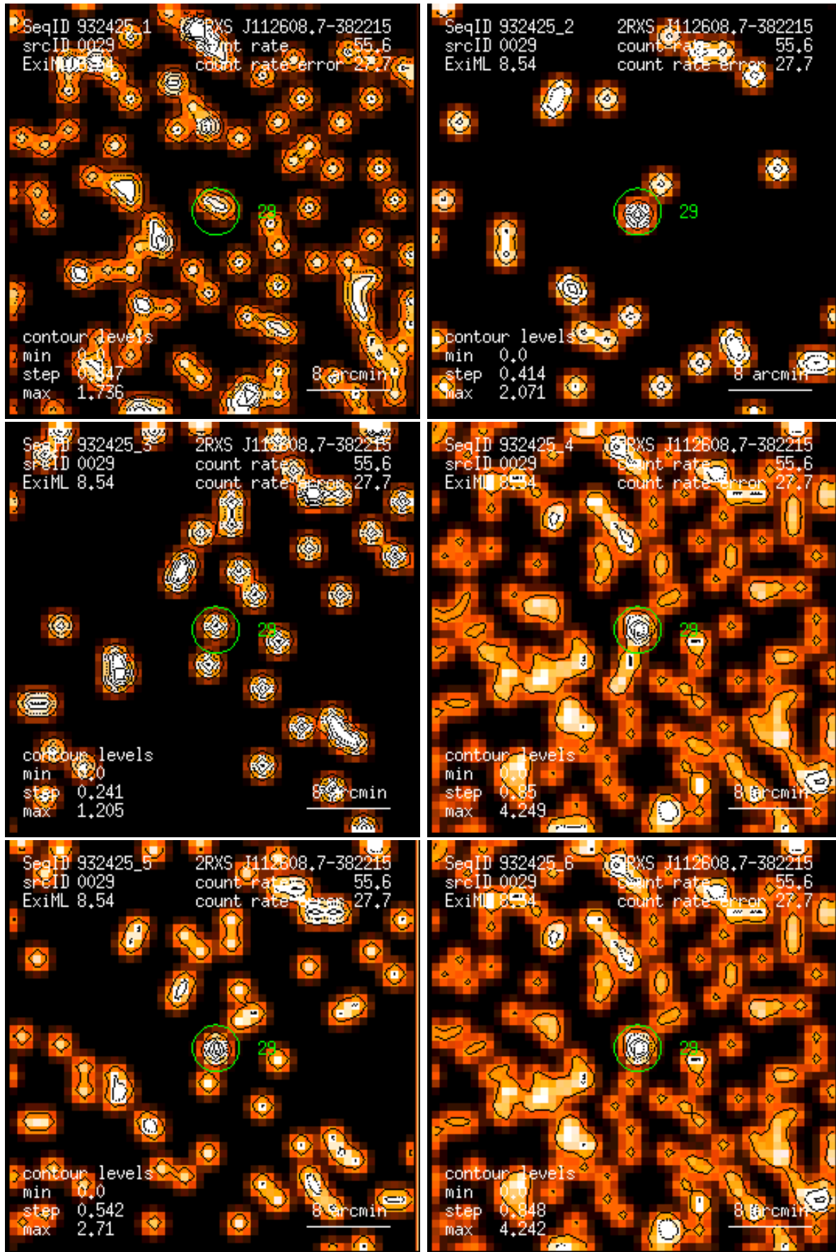
Figure 29: RASS 932425: detection 0029: band rate images, Gaussian filter: (1) PSPC channels 11 – 41, (2) 52 – 90, (3) 91 – 201, (4) 11 – 235, (5) 52 – 201, (6) 11 – 201. Broad band rates in counts/ks. Band rate contour levels in counts/ks/arcmin 2 .
