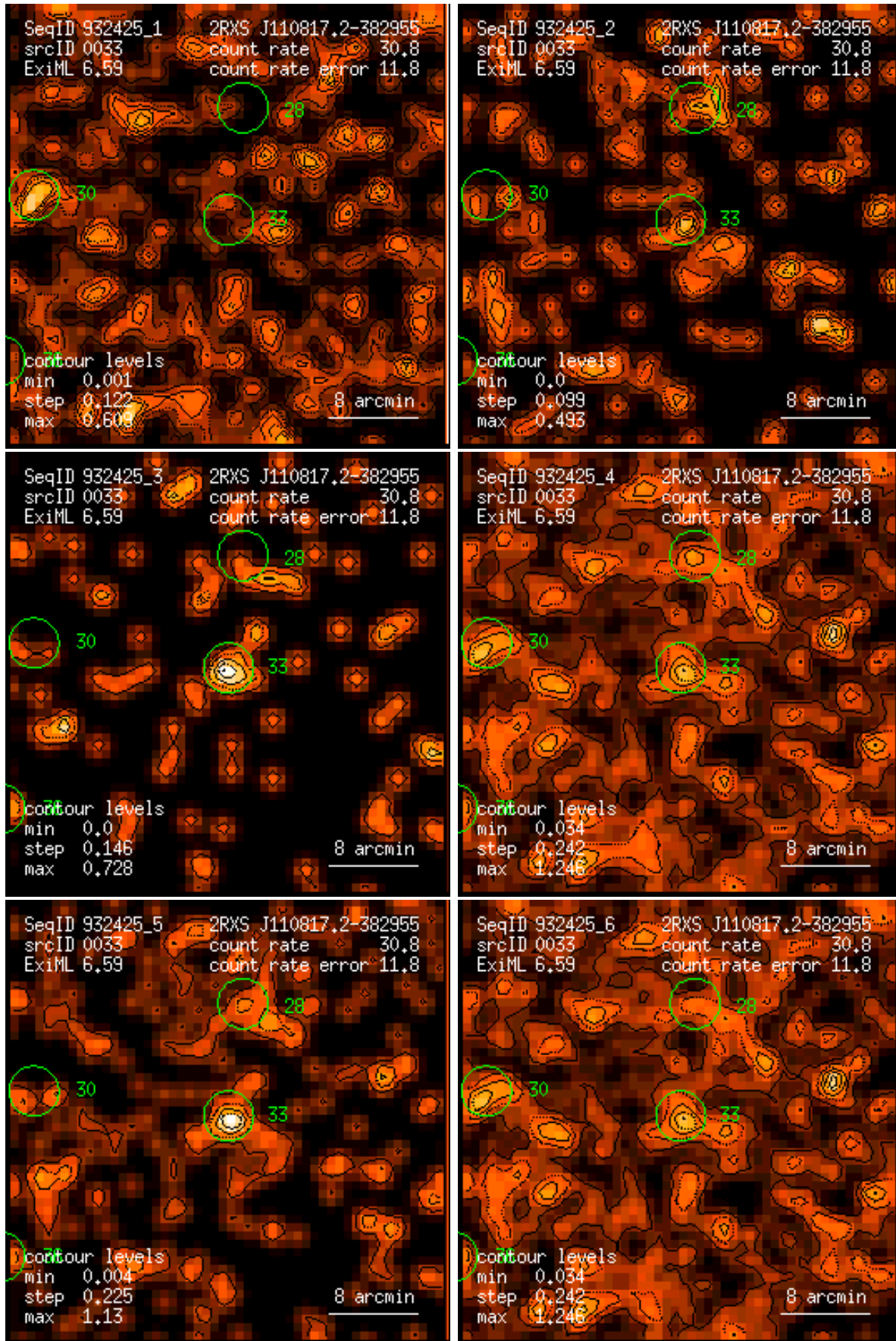
Figure 33: RASS 932425: detection 0033: band rate images, Gaussian filter: (1) PSPC channels 11 – 41, (2) 52 – 90, (3) 91 – 201, (4) 11 – 235, (5) 52 – 201, (6) 11 – 201. Broad band rates in counts/ks. Band rate contour levels in counts/ks/arcmin 2 .
