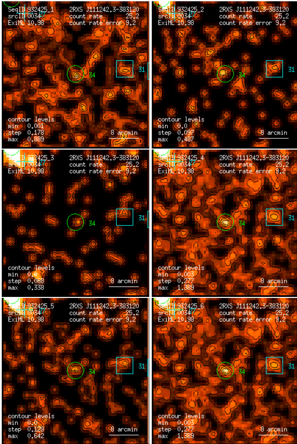
Figure 34: RASS 932425: detection 0034: band rate images, Gaussian filter: (1) PSPC channels 11 – 41, (2) 52 – 90, (3) 91 – 201, (4) 11 – 235, (5) 52 – 201, (6) 11 – 201. Broad band rates in counts/ks. Band rate contour levels in counts/ks/arcmin 2 .
