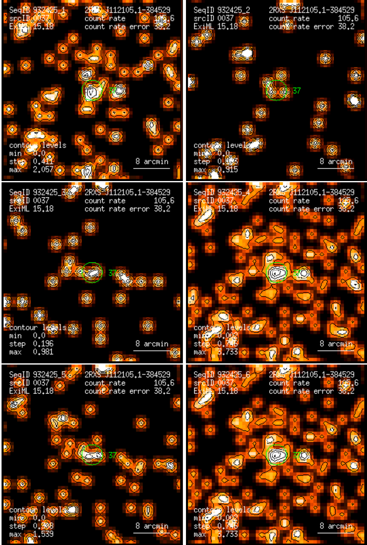
Figure 37: RASS 932425: detection 0037: band rate images, Gaussian filter: (1) PSPC channels 11 – 41, (2) 52 – 90, (3) 91 – 201, (4) 11 – 235, (5) 52 – 201, (6) 11 – 201. Broad band rates in counts/ks. Band rate contour levels in counts/ks/arcmin 2 .
