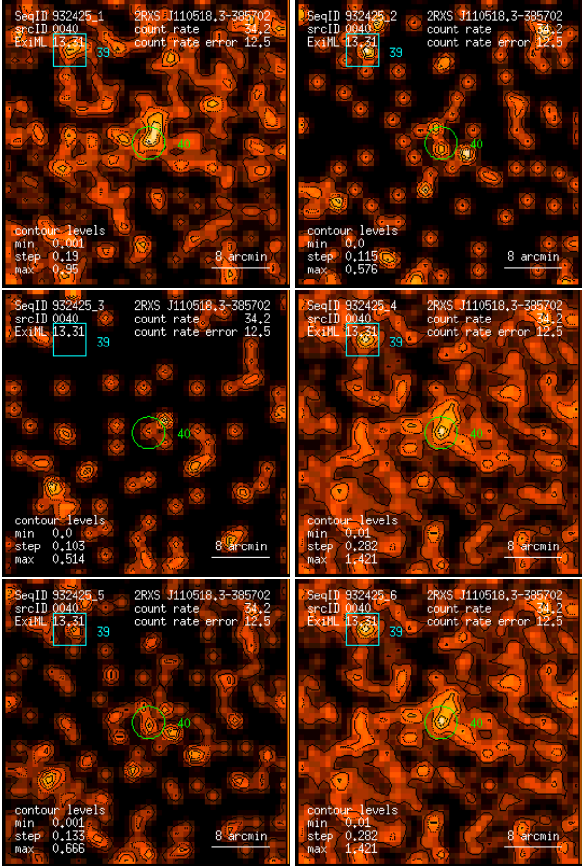
Figure 40: RASS 932425: detection 0040: band rate images, Gaussian filter: (1) PSPC channels 11 – 41, (2) 52 – 90, (3) 91 – 201, (4) 11 – 235, (5) 52 – 201, (6) 11 – 201. Broad band rates in counts/ks. Band rate contour levels in counts/ks/arcmin 2 .
