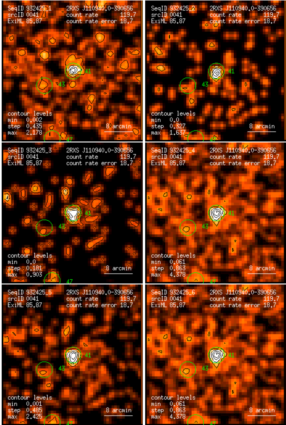
Figure 41: RASS 932425: detection 0041: band rate images, Gaussian filter: (1) PSPC channels 11 – 41, (2) 52 – 90, (3) 91 – 201, (4) 11 – 235, (5) 52 – 201, (6) 11 – 201. Broad band rates in counts/ks. Band rate contour levels in counts/ks/arcmin 2 .
