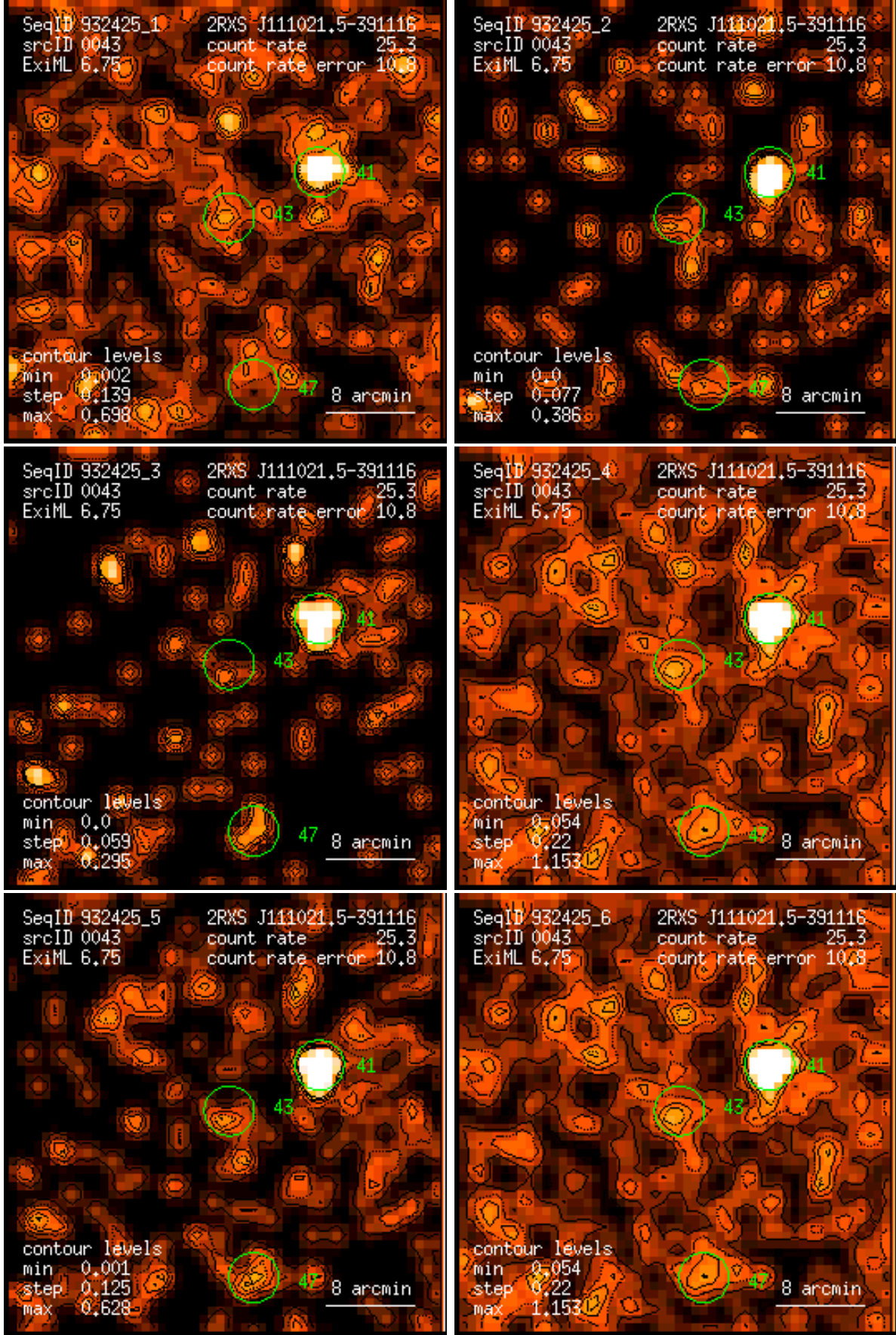
Figure 43: RASS 932425: detection 0043: band rate images, Gaussian filter: (1) PSPC channels 11 – 41, (2) 52 – 90, (3) 91 – 201, (4) 11 – 235, (5) 52 – 201, (6) 11 – 201. Broad band rates in counts/ks. Band rate contour levels in counts/ks/arcmin 2 .
