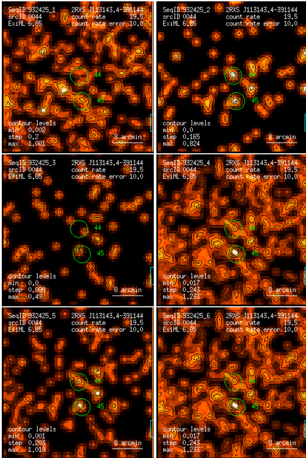
Figure 44: RASS 932425: detection 0044: band rate images, Gaussian filter: (1) PSPC channels 11 – 41, (2) 52 – 90, (3) 91 – 201, (4) 11 – 235, (5) 52 – 201, (6) 11 – 201. Broad band rates in counts/ks. Band rate contour levels in counts/ks/arcmin 2 .
