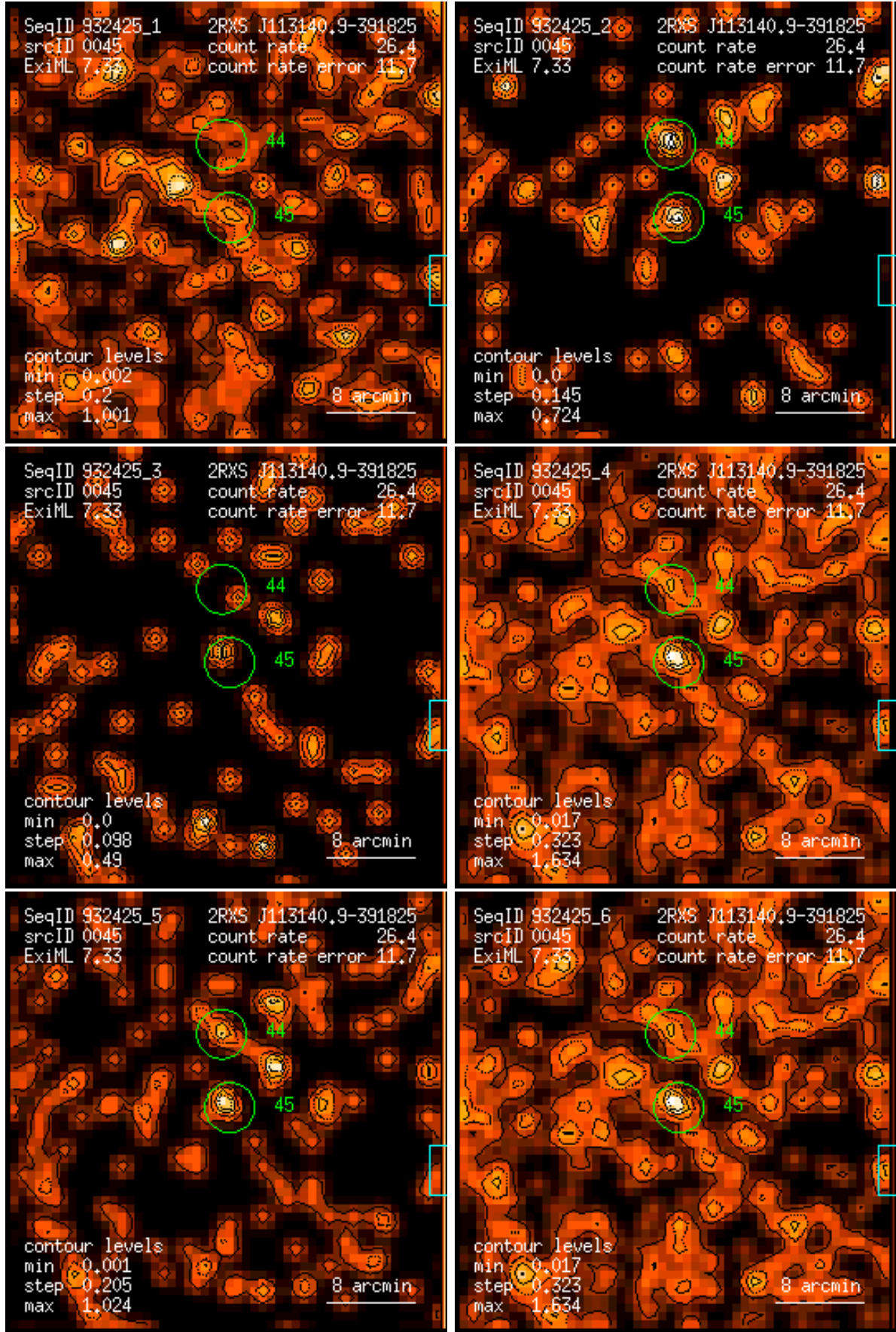
Figure 45: RASS 932425: detection 0045: band rate images, Gaussian filter: (1) PSPC channels 11 – 41, (2) 52 – 90, (3) 91 – 201, (4) 11 – 235, (5) 52 – 201, (6) 11 – 201. Broad band rates in counts/ks. Band rate contour levels in counts/ks/arcmin 2 .
