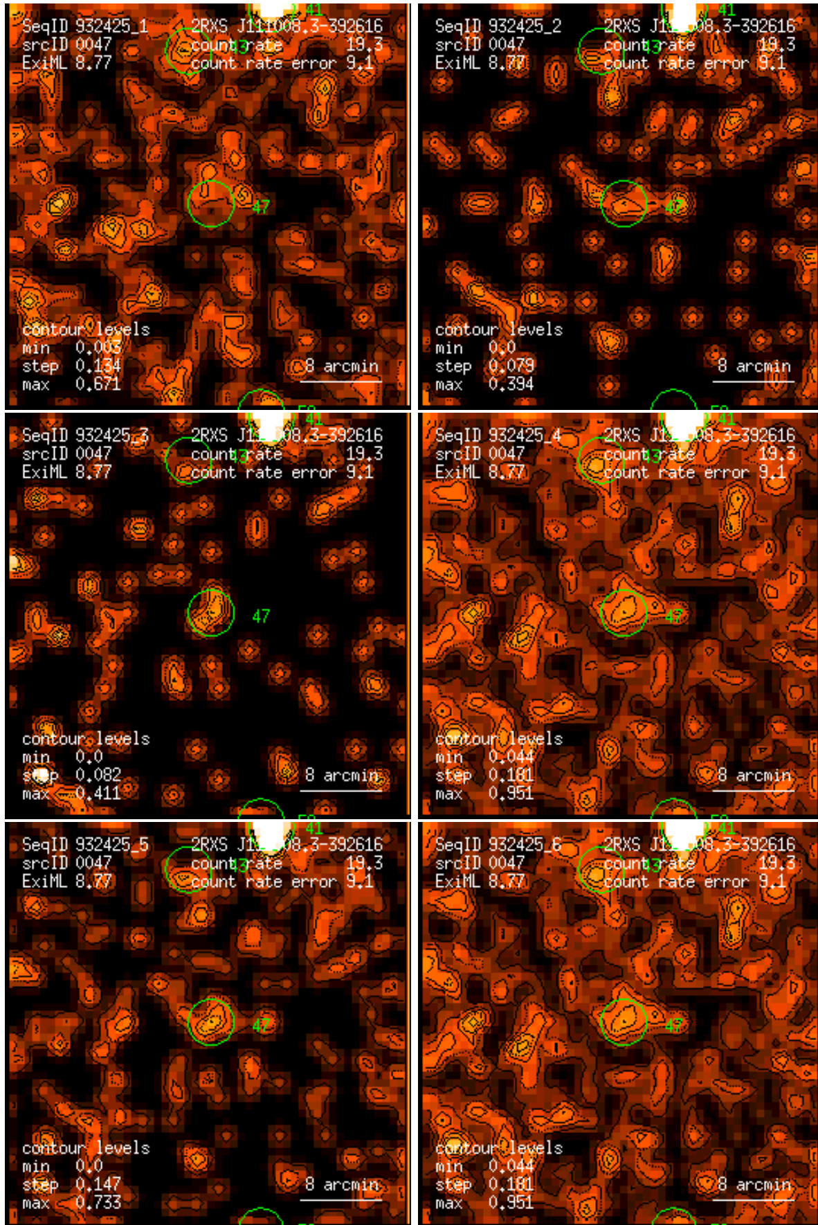
Figure 47: RASS 932425: detection 0047: band rate images, Gaussian filter: (1) PSPC channels 11 – 41, (2) 52 – 90, (3) 91 – 201, (4) 11 – 235, (5) 52 – 201, (6) 11 – 201. Broad band rates in counts/ks. Band rate contour levels in counts/ks/arcmin 2 .
