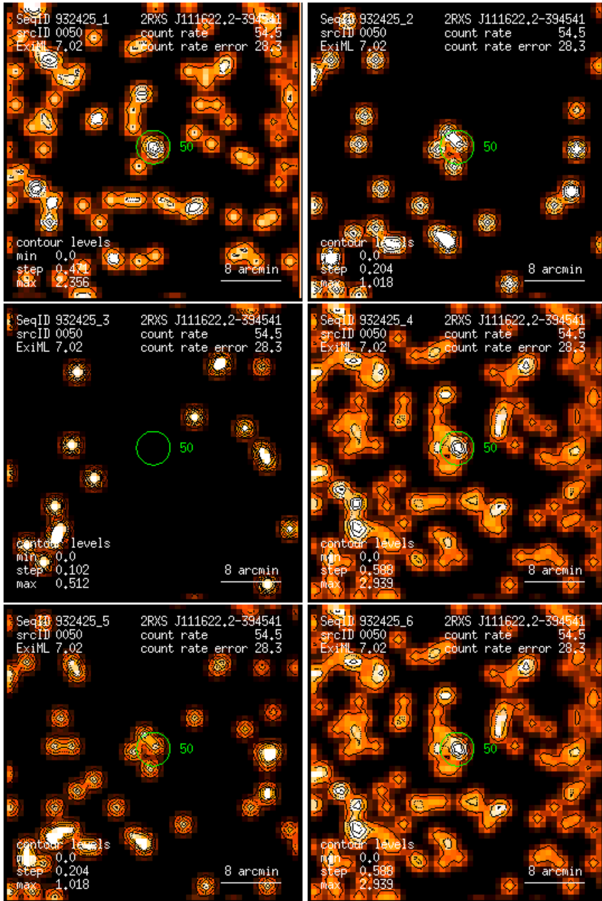
Figure 50: RASS 932425: detection 0050: band rate images, Gaussian filter: (1) PSPC channels 11 – 41, (2) 52 – 90, (3) 91 – 201, (4) 11 – 235, (5) 52 – 201, (6) 11 – 201. Broad band rates in counts/ks. Band rate contour levels in counts/ks/arcmin 2 .
