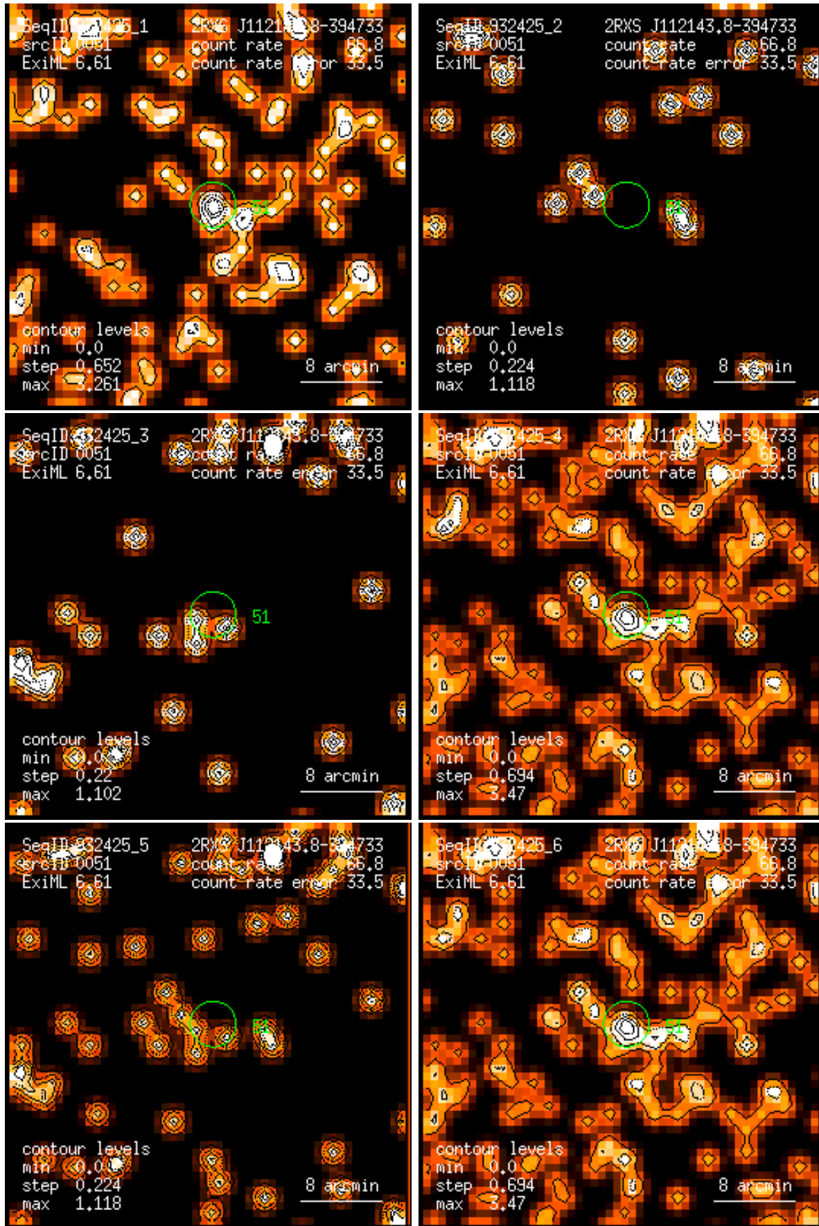
Figure 51: RASS 932425: detection 0051: band rate images, Gaussian filter: (1) PSPC channels 11 – 41, (2) 52 – 90, (3) 91 – 201, (4) 11 – 235, (5) 52 – 201, (6) 11 – 201. Broad band rates in counts/ks. Band rate contour levels in counts/ks/arcmin 2 .
