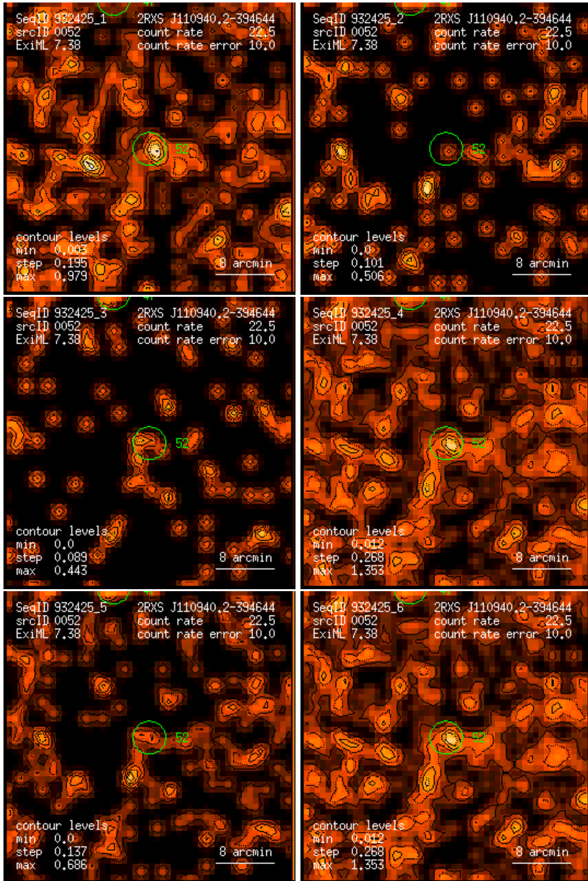
Figure 52: RASS 932425: detection 0052: band rate images, Gaussian filter: (1) PSPC channels 11 – 41, (2) 52 – 90, (3) 91 – 201, (4) 11 – 235, (5) 52 – 201, (6) 11 – 201. Broad band rates in counts/ks. Band rate contour levels in counts/ks/arcmin 2 .
