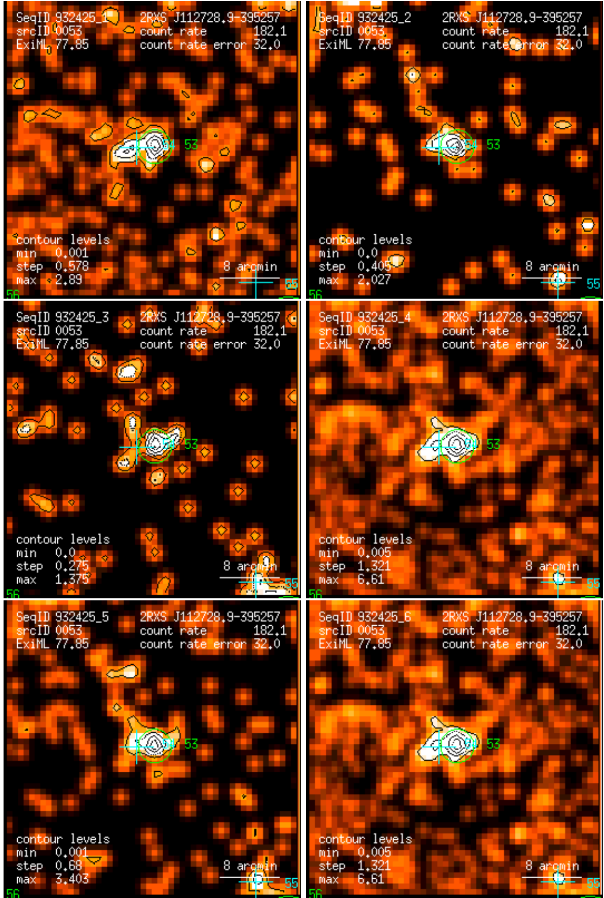
Figure 53: RASS 932425: detection 0053: band rate images, Gaussian filter: (1) PSPC channels 11 – 41, (2) 52 – 90, (3) 91 – 201, (4) 11 – 235, (5) 52 – 201, (6) 11 – 201. Broad band rates in counts/ks. Band rate contour levels in counts/ks/arcmin 2 .
