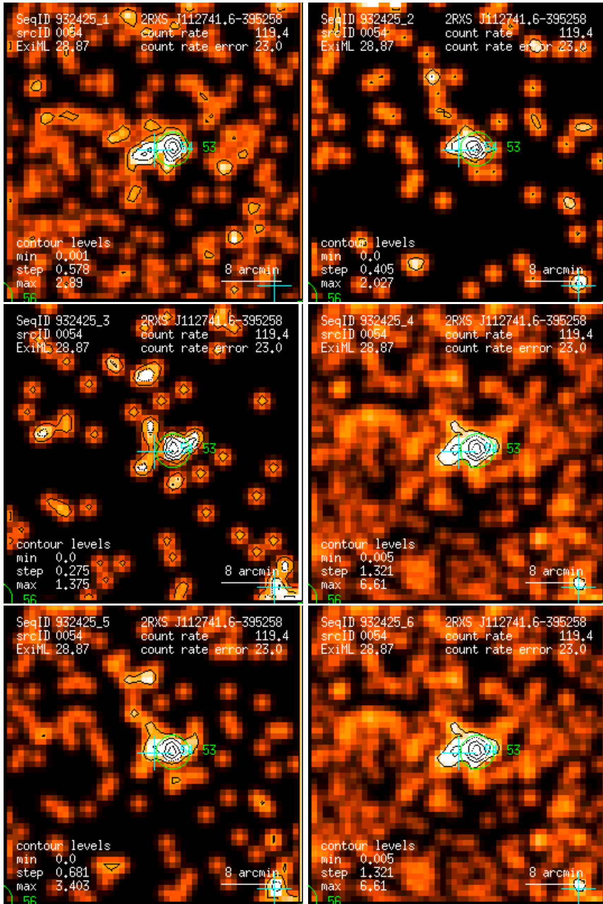
Figure 54: RASS 932425: detection 0054: band rate images, Gaussian filter: (1) PSPC channels 11 – 41, (2) 52 – 90, (3) 91 – 201, (4) 11 – 235, (5) 52 – 201, (6) 11 – 201. Broad band rates in counts/ks. Band rate contour levels in counts/ks/arcmin 2 .
