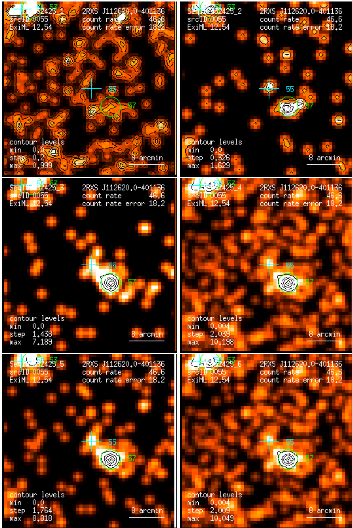
Figure 55: RASS 932425: detection 0055: band rate images, Gaussian filter: (1) PSPC channels 11 – 41, (2) 52 – 90, (3) 91 – 201, (4) 11 – 235, (5) 52 – 201, (6) 11 – 201. Broad band rates in counts/ks. Band rate contour levels in counts/ks/arcmin 2 .
