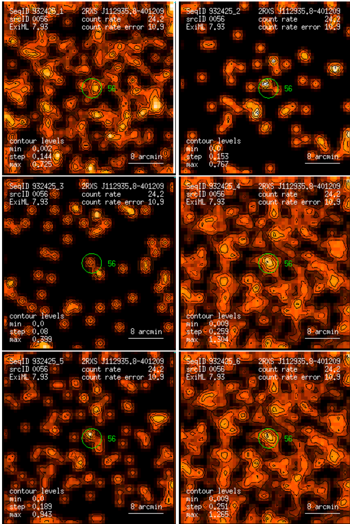
Figure 56: RASS 932425: detection 0056: band rate images, Gaussian filter: (1) PSPC channels 11 – 41, (2) 52 – 90, (3) 91 – 201, (4) 11 – 235, (5) 52 – 201, (6) 11 – 201. Broad band rates in counts/ks. Band rate contour levels in counts/ks/arcmin 2 .
