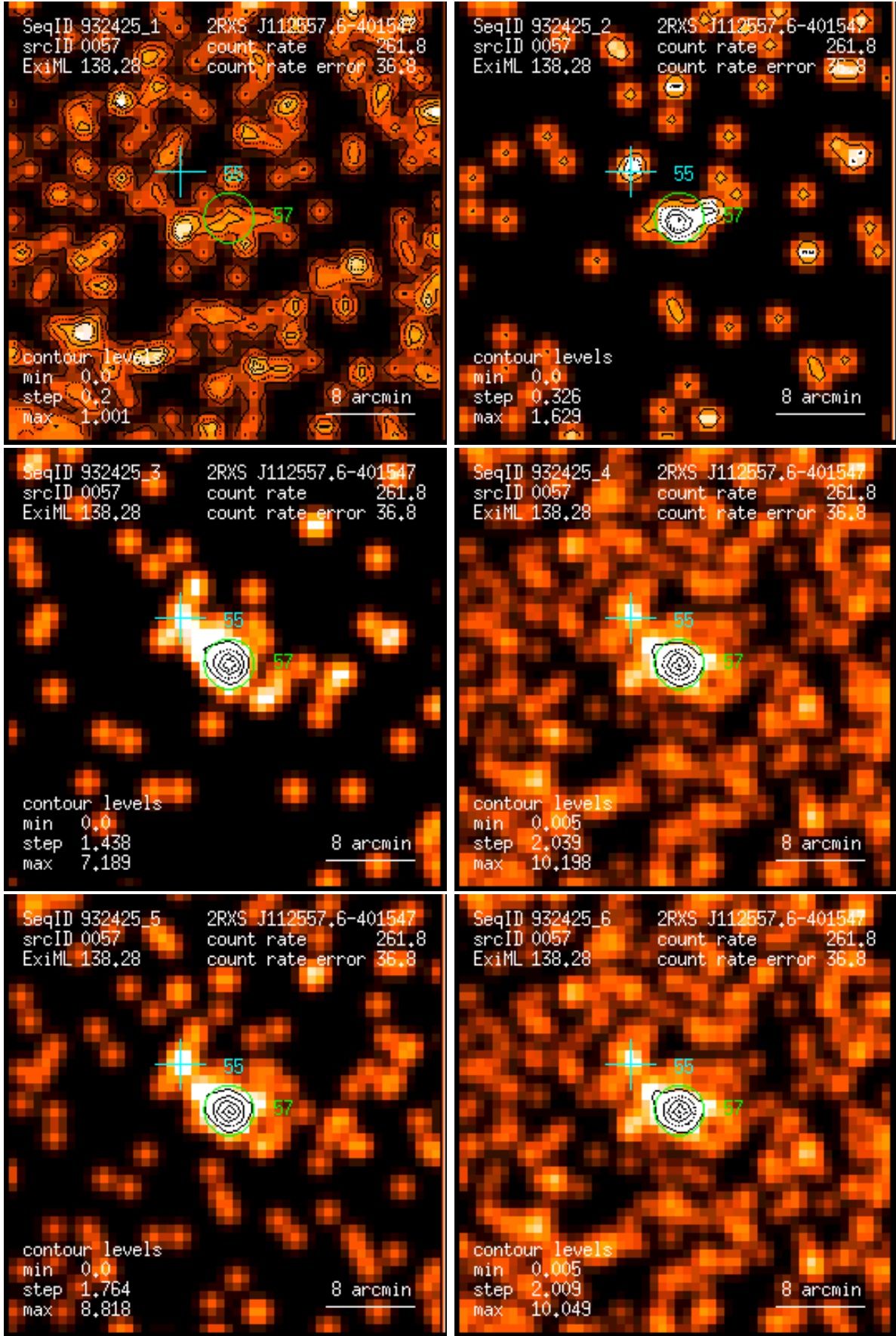
Figure 57: RASS 932425: detection 0057: band rate images, Gaussian filter: (1) PSPC channels 11 – 41, (2) 52 – 90, (3) 91 – 201, (4) 11 – 235, (5) 52 – 201, (6) 11 – 201. Broad band rates in counts/ks. Band rate contour levels in counts/ks/arcmin 2 .
