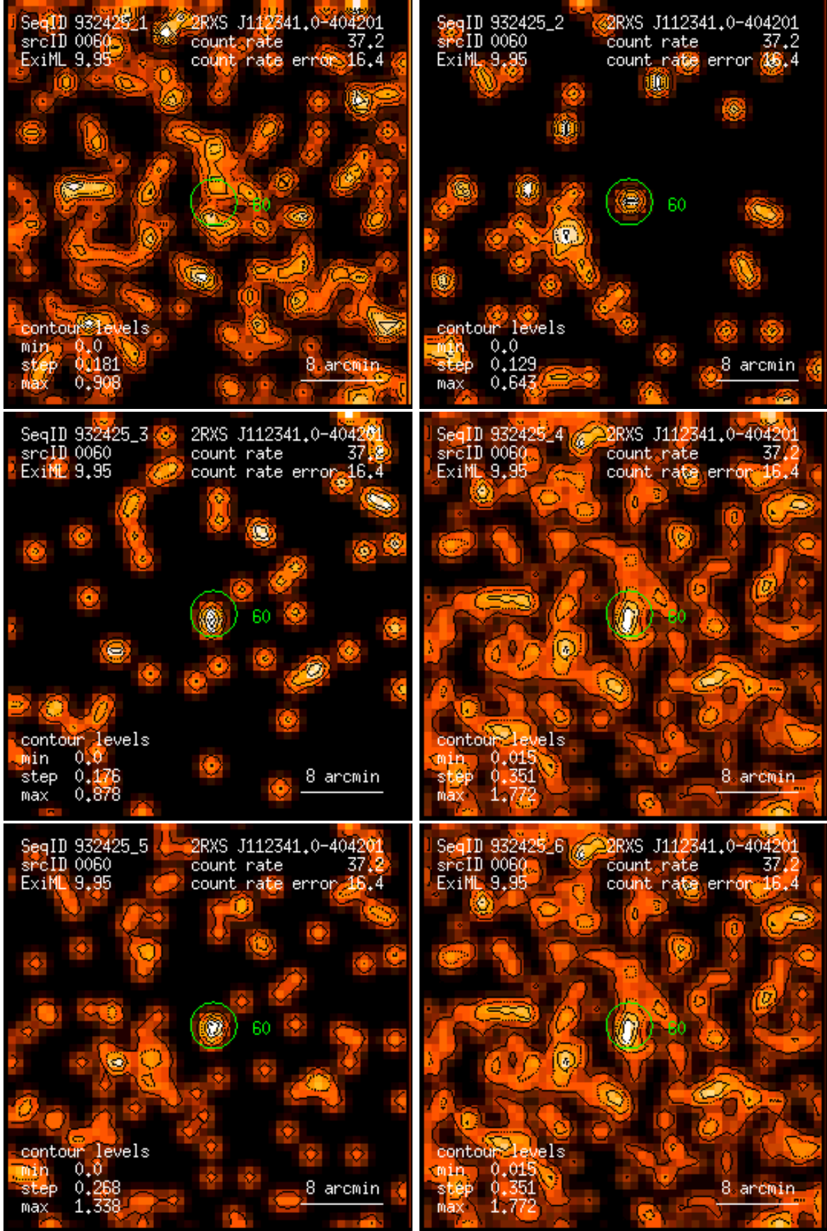
Figure 60: RASS 932425: detection 0060: band rate images, Gaussian filter: (1) PSPC channels 11 – 41, (2) 52 – 90, (3) 91 – 201, (4) 11 – 235, (5) 52 – 201, (6) 11 – 201. Broad band rates in counts/ks. Band rate contour levels in counts/ks/arcmin 2 .
