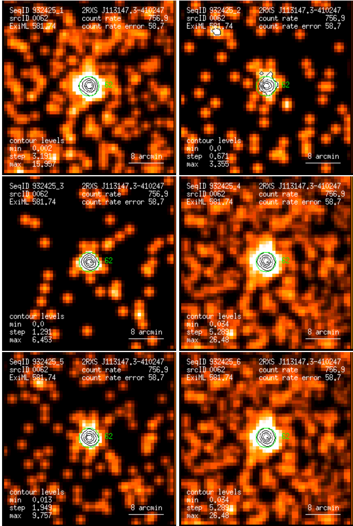
Figure 62: RASS 932425: detection 0062: band rate images, Gaussian filter: (1) PSPC channels 11 – 41, (2) 52 – 90, (3) 91 – 201, (4) 11 – 235, (5) 52 – 201, (6) 11 – 201. Broad band rates in counts/ks. Band rate contour levels in counts/ks/arcmin 2 .
