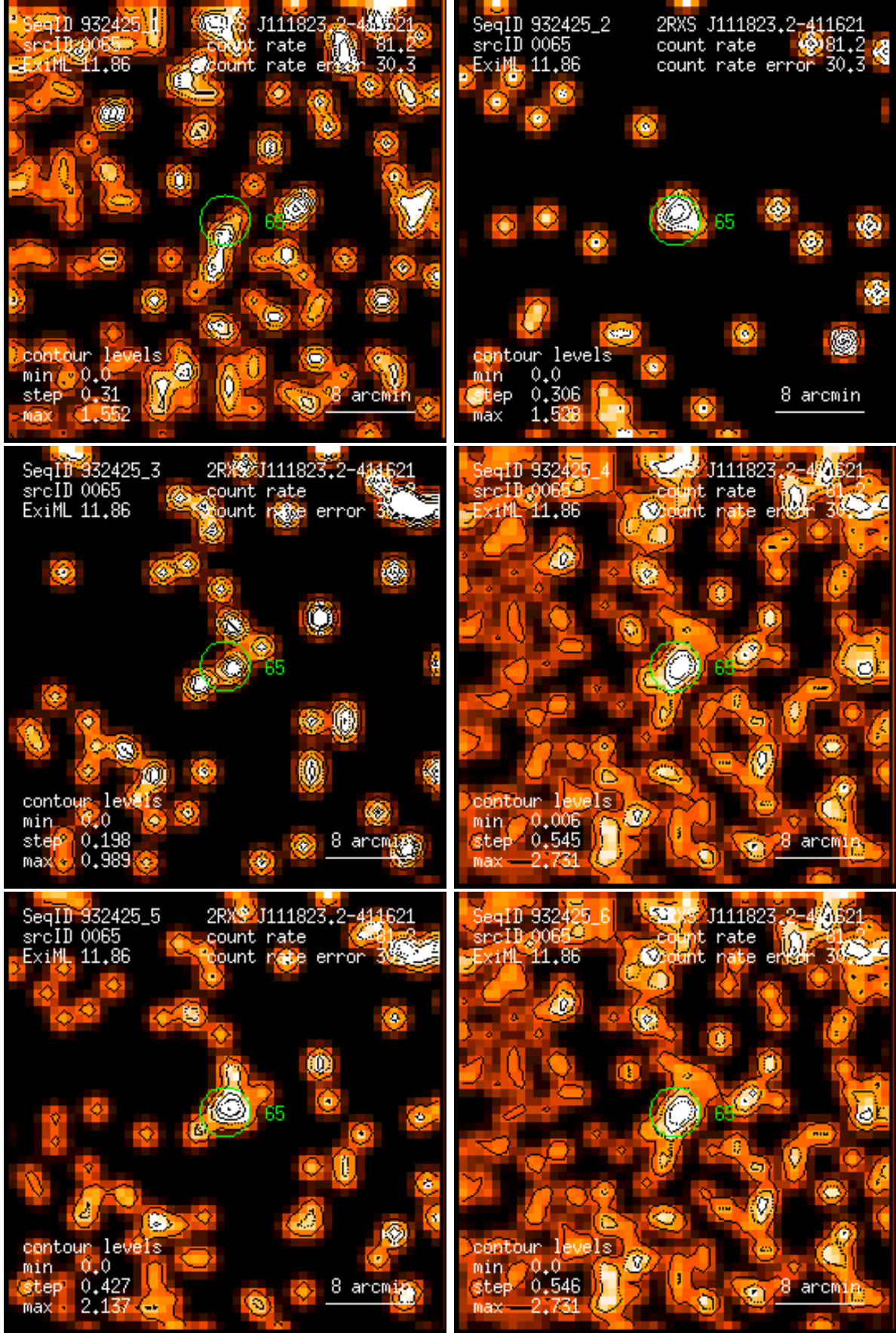
Figure 65: RASS 932425: detection 0065: band rate images, Gaussian filter: (1) PSPC channels 11 – 41, (2) 52 – 90, (3) 91 – 201, (4) 11 – 235, (5) 52 – 201, (6) 11 – 201. Broad band rates in counts/ks. Band rate contour levels in counts/ks/arcmin 2 .
