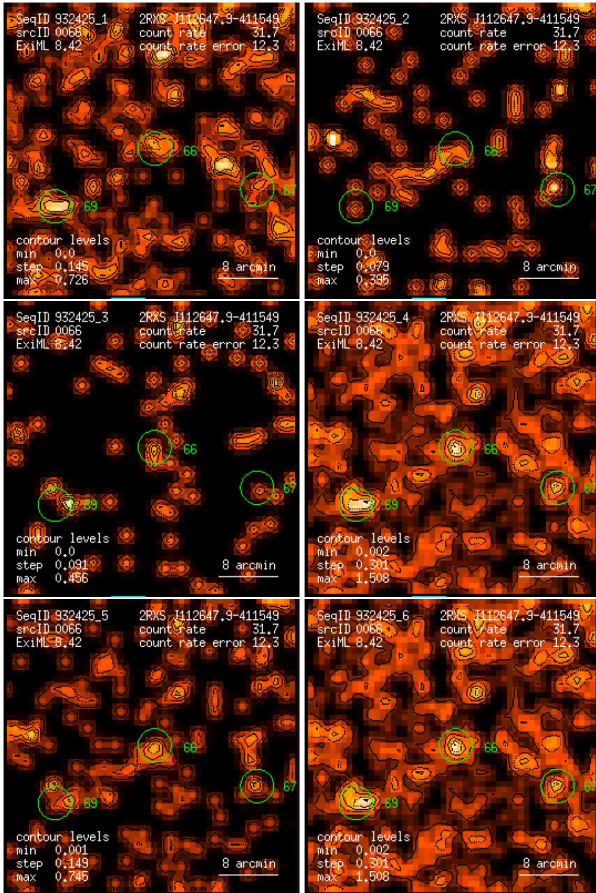
Figure 66: RASS 932425: detection 0066: band rate images, Gaussian filter: (1) PSPC channels 11 – 41, (2) 52 – 90, (3) 91 – 201, (4) 11 – 235, (5) 52 – 201, (6) 11 – 201. Broad band rates in counts/ks. Band rate contour levels in counts/ks/arcmin 2 .
