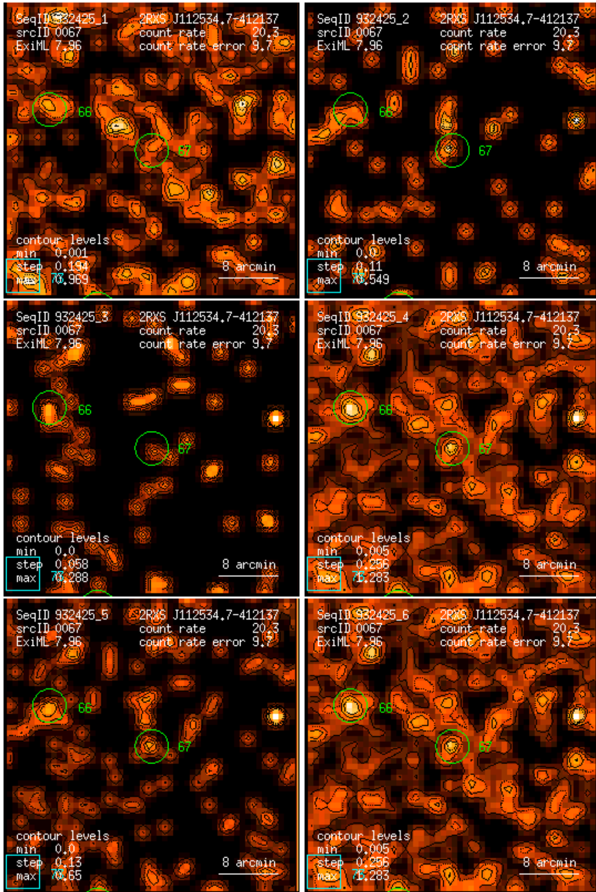
Figure 67: RASS 932425: detection 0067: band rate images, Gaussian filter: (1) PSPC channels 11 – 41, (2) 52 – 90, (3) 91 – 201, (4) 11 – 235, (5) 52 – 201, (6) 11 – 201. Broad band rates in counts/ks. Band rate contour levels in counts/ks/arcmin 2 .
