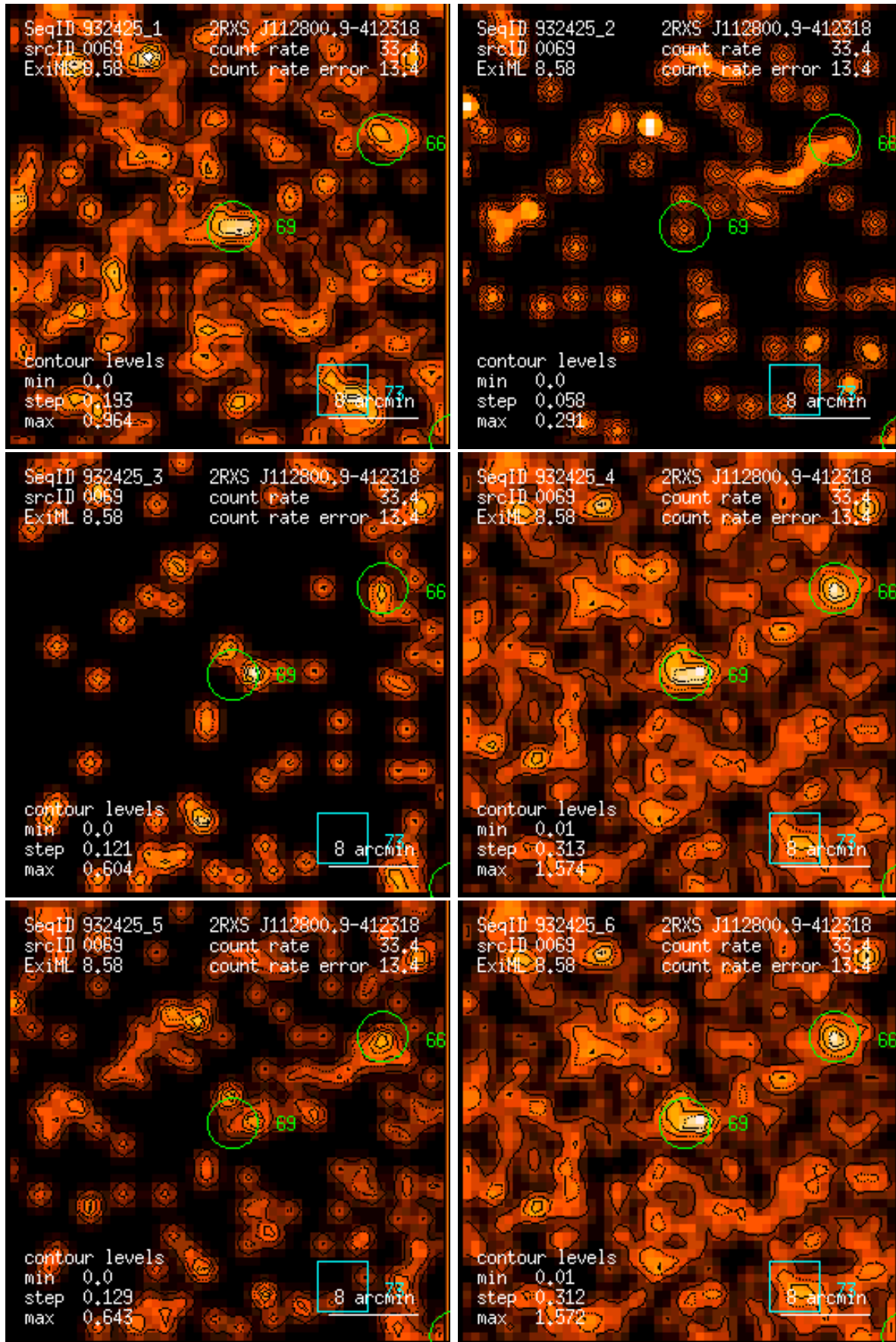
Figure 69: RASS 932425: detection 0069: band rate images, Gaussian filter: (1) PSPC channels 11 – 41, (2) 52 – 90, (3) 91 – 201, (4) 11 – 235, (5) 52 – 201, (6) 11 – 201. Broad band rates in counts/ks. Band rate contour levels in counts/ks/arcmin 2 .
