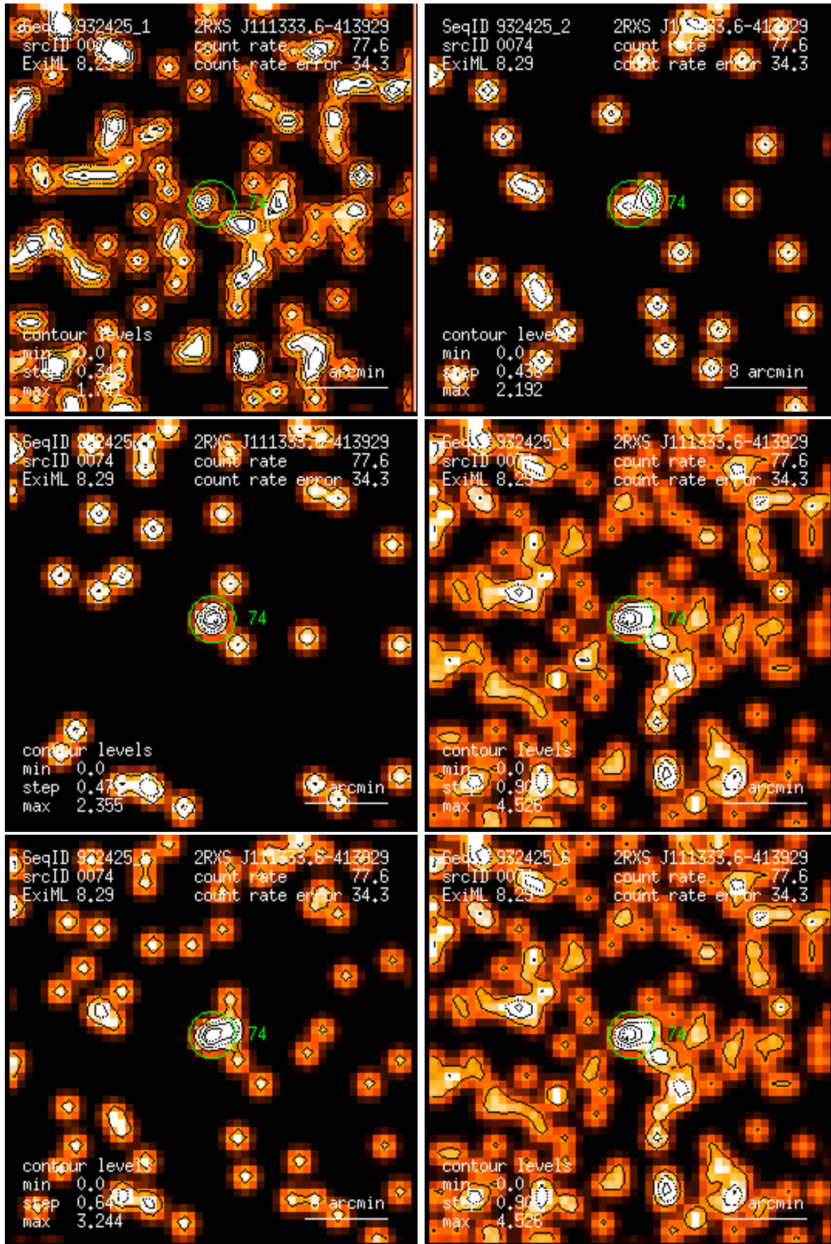
Figure 74: RASS 932425: detection 0074: band rate images, Gaussian filter: (1) PSPC channels 11 – 41, (2) 52 – 90, (3) 91 – 201, (4) 11 – 235, (5) 52 – 201, (6) 11 – 201. Broad band rates in counts/ks. Band rate contour levels in counts/ks/arcmin 2 .
