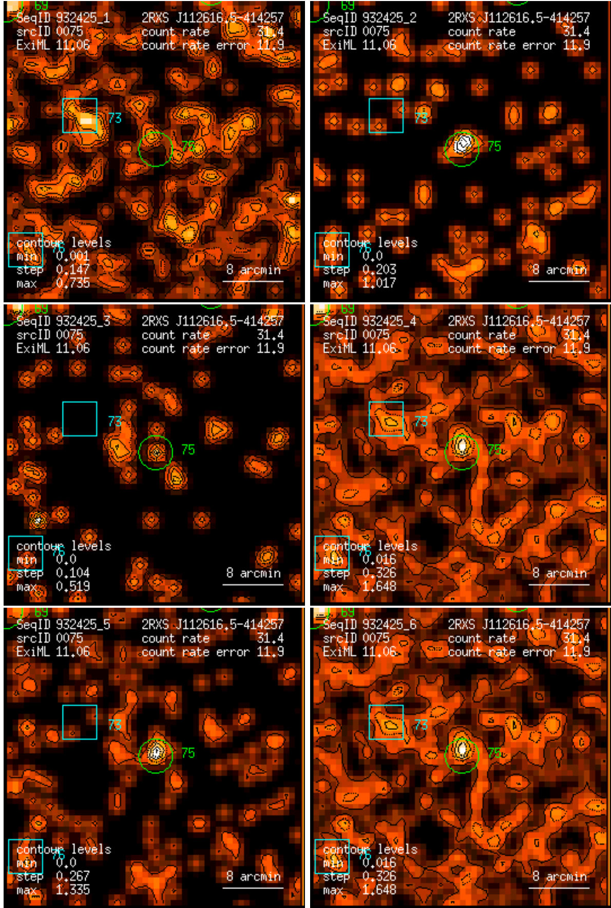
Figure 75: RASS 932425: detection 0075: band rate images, Gaussian filter: (1) PSPC channels 11 – 41, (2) 52 – 90, (3) 91 – 201, (4) 11 – 235, (5) 52 – 201, (6) 11 – 201. Broad band rates in counts/ks. Band rate contour levels in counts/ks/arcmin 2 .
