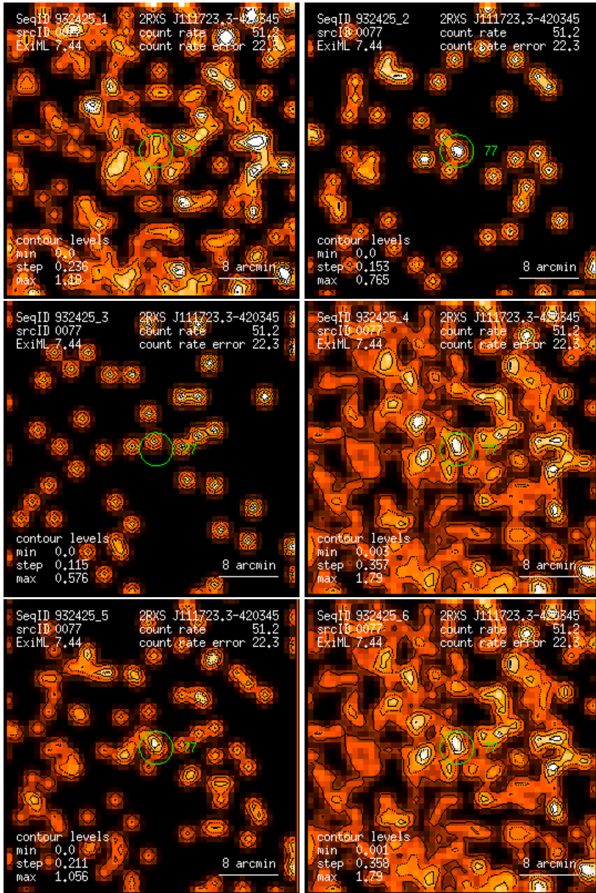
Figure 77: RASS 932425: detection 0077: band rate images, Gaussian filter: (1) PSPC channels 11 – 41, (2) 52 – 90, (3) 91 – 201, (4) 11 – 235, (5) 52 – 201, (6) 11 – 201. Broad band rates in counts/ks. Band rate contour levels in counts/ks/arcmin 2 .
