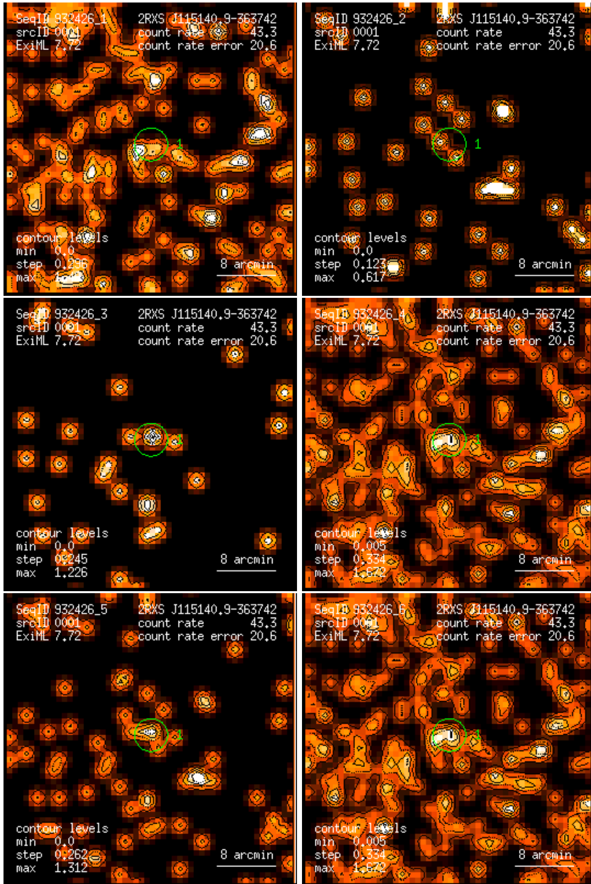
Figure 1: RASS 932426: detection 0001: band rate images, Gaussian filter: (1) PSPC channels 11 – 41, (2) 52 – 90, (3) 91 – 201, (4) 11 – 235, (5) 52 – 201, (6) 11 – 201. Broad band rates in counts/ks. Band rate contour levels in counts/ks/arcmin 2 .
