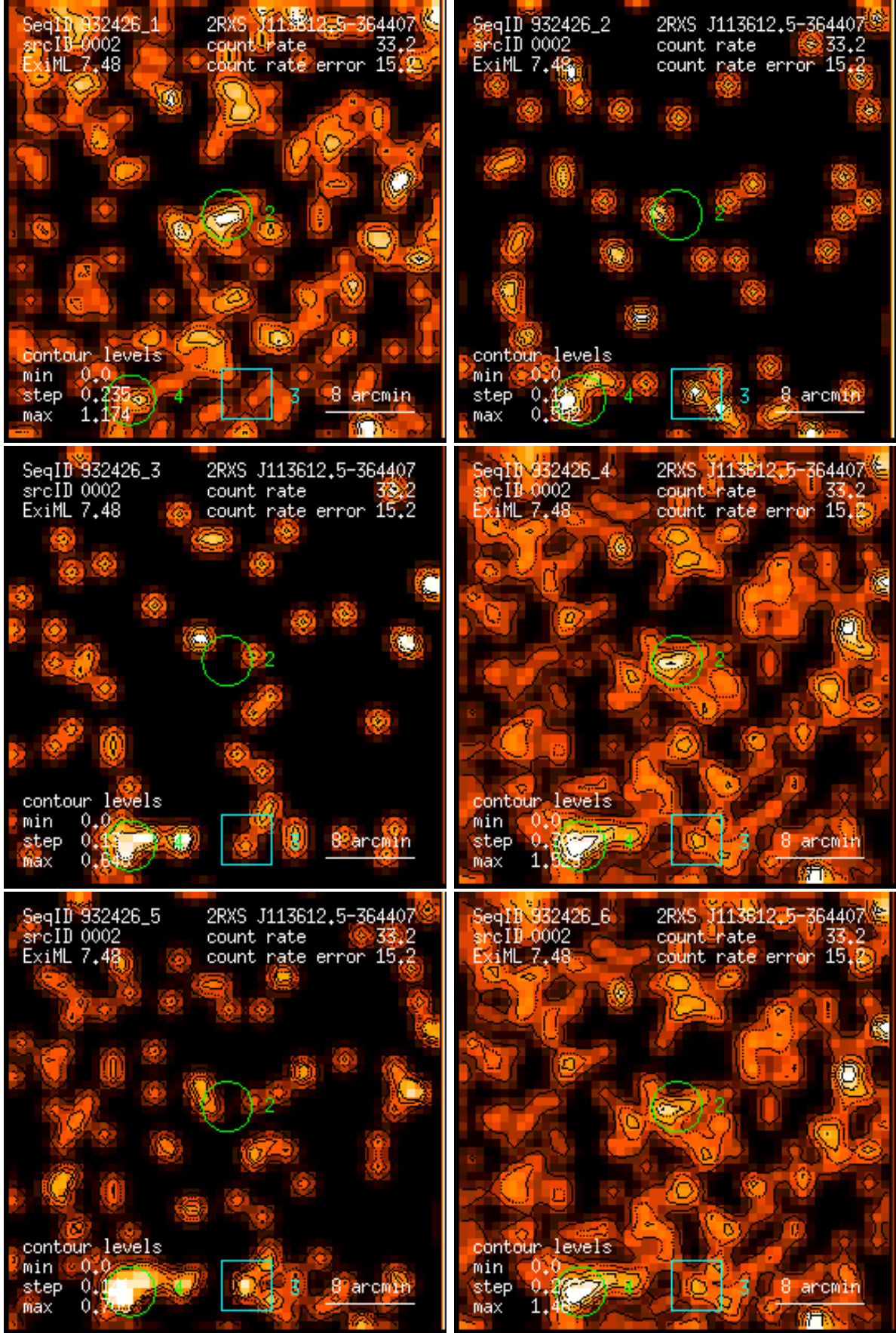
Figure 2: RASS 932426: detection 0002: band rate images, Gaussian filter: (1) PSPC channels 11 – 41, (2) 52 – 90, (3) 91 – 201, (4) 11 – 235, (5) 52 – 201, (6) 11 – 201. Broad band rates in counts/ks. Band rate contour levels in counts/ks/arcmin 2 .
