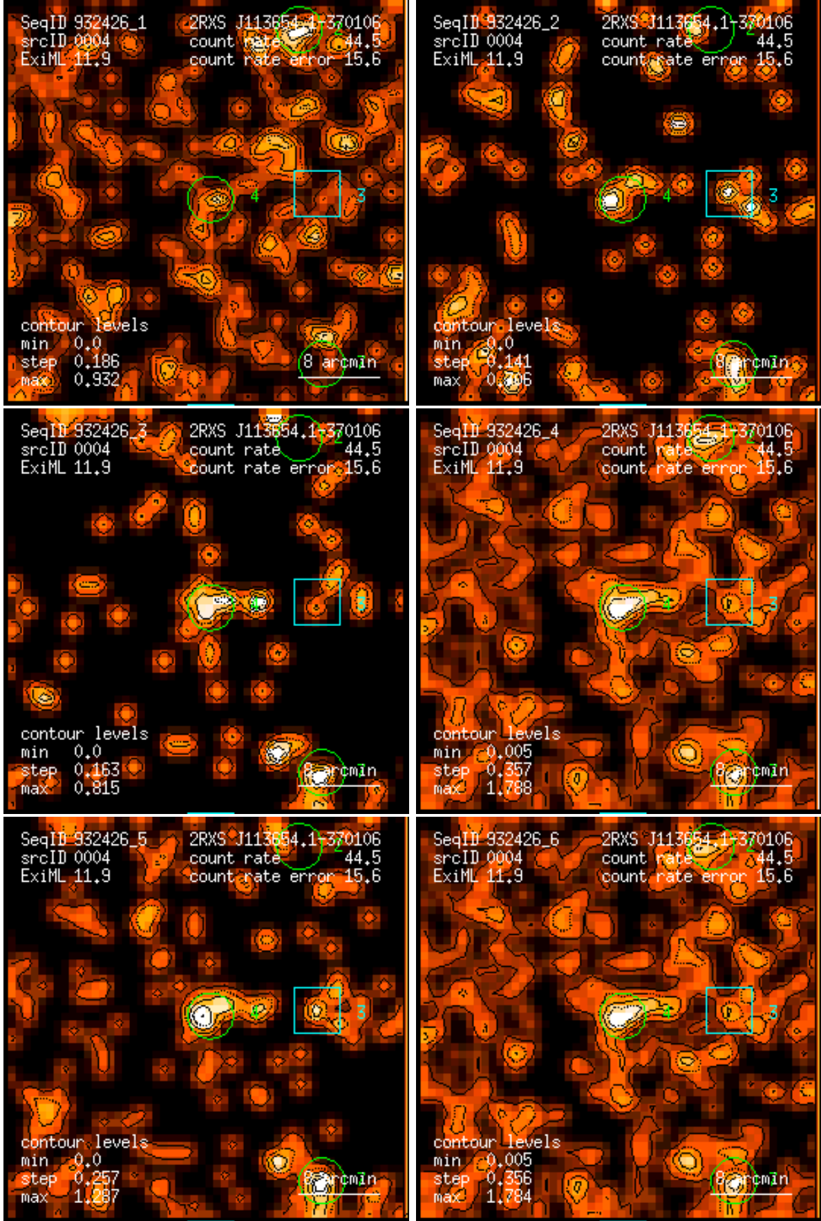
Figure 4: RASS 932426: detection 0004: band rate images, Gaussian filter: (1) PSPC channels 11 – 41, (2) 52 – 90, (3) 91 – 201, (4) 11 – 235, (5) 52 – 201, (6) 11 – 201. Broad band rates in counts/ks. Band rate contour levels in counts/ks/arcmin 2 .
