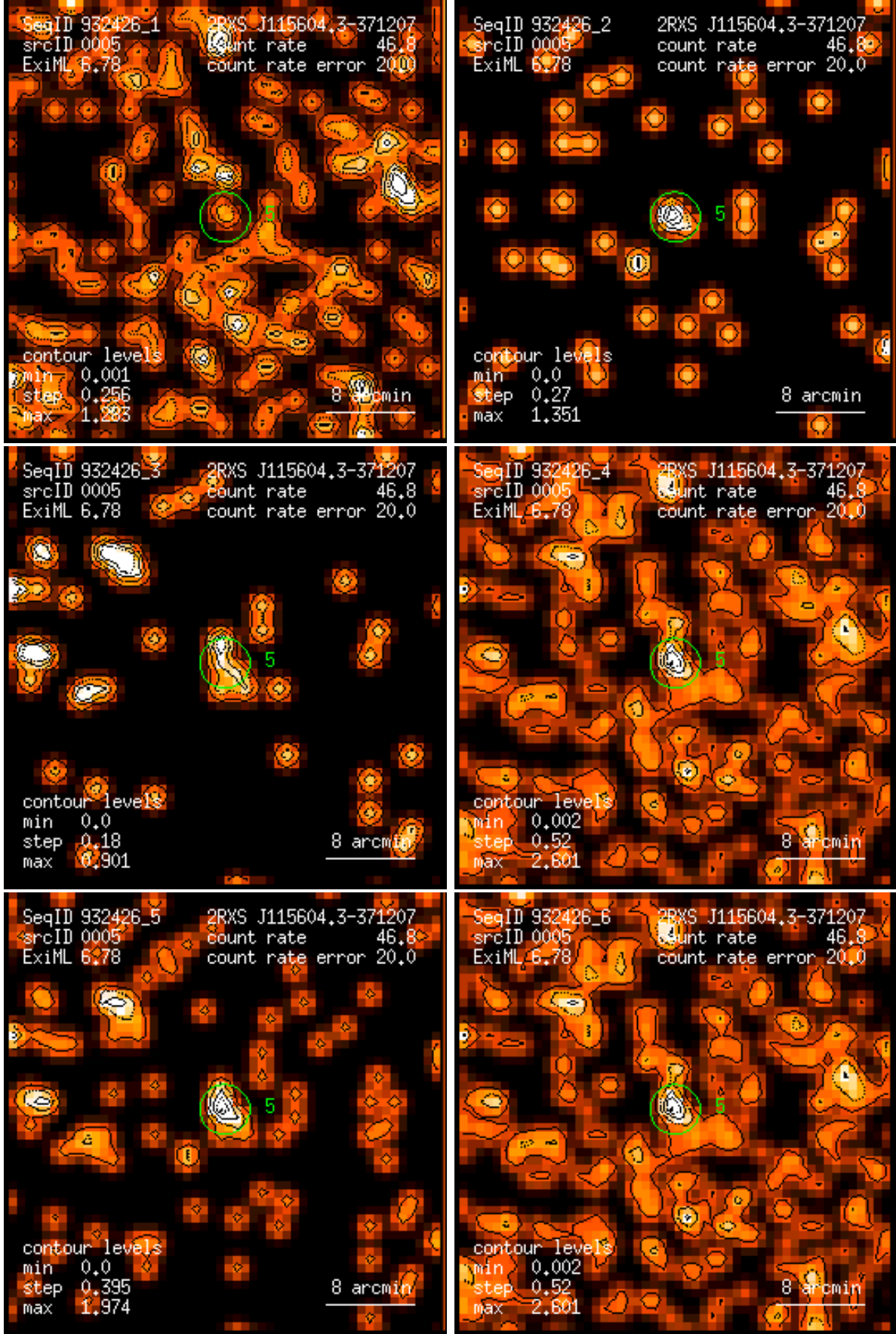
Figure 5: RASS 932426: detection 0005: band rate images, Gaussian filter: (1) PSPC channels 11 – 41, (2) 52 – 90, (3) 91 – 201, (4) 11 – 235, (5) 52 – 201, (6) 11 – 201. Broad band rates in counts/ks. Band rate contour levels in counts/ks/arcmin 2 .
