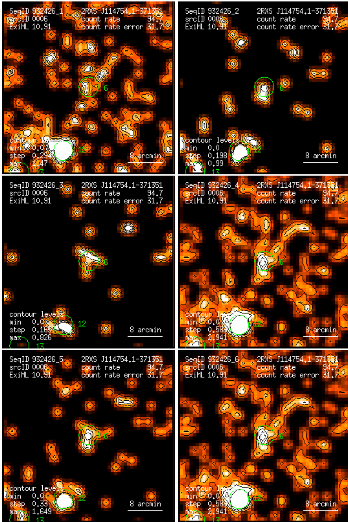
Figure 6: RASS 932426: detection 0006: band rate images, Gaussian filter: (1) PSPC channels 11 – 41, (2) 52 – 90, (3) 91 – 201, (4) 11 – 235, (5) 52 – 201, (6) 11 – 201. Broad band rates in counts/ks. Band rate contour levels in counts/ks/arcmin 2 .
