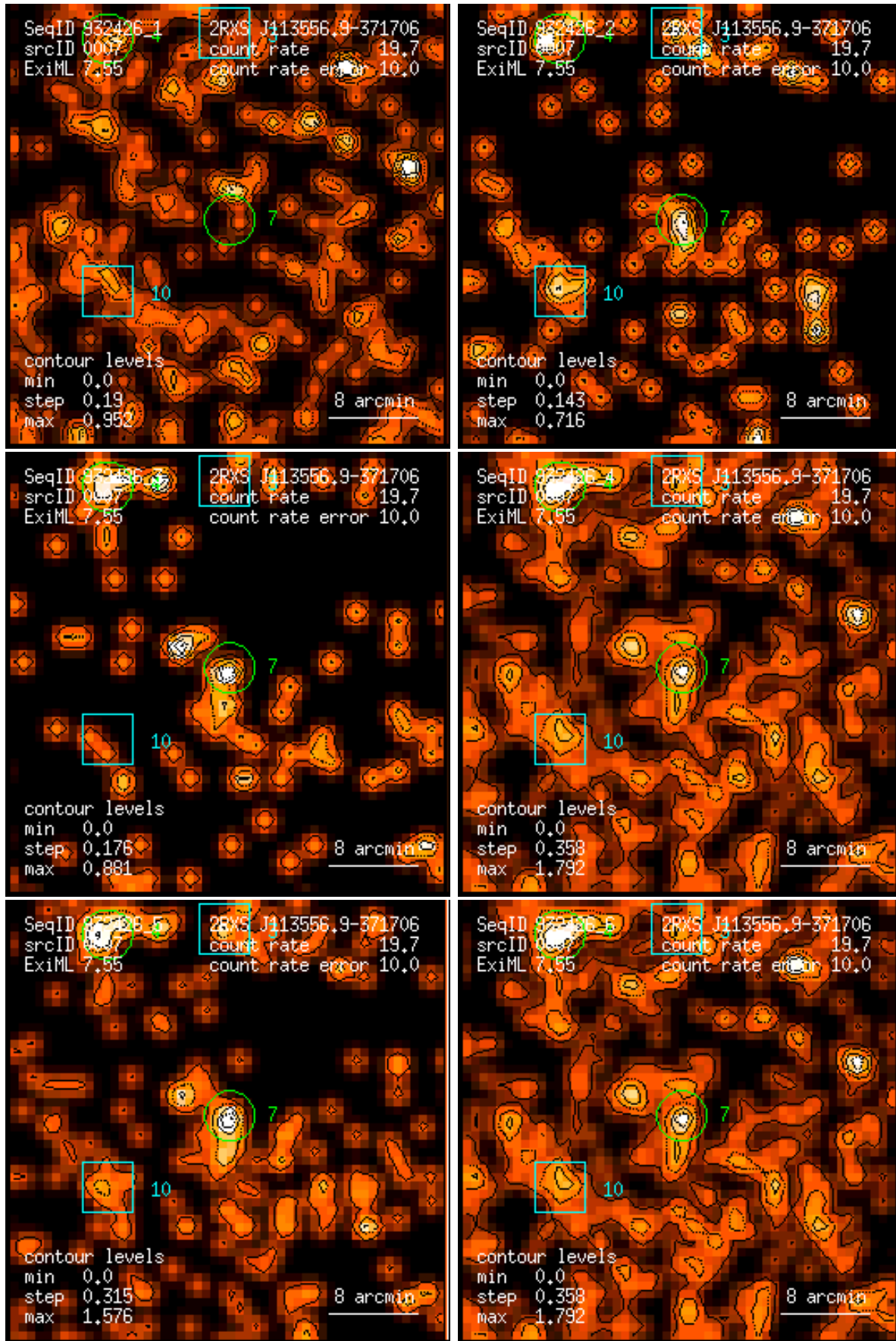
Figure 7: RASS 932426: detection 0007: band rate images, Gaussian filter: (1) PSPC channels 11 – 41, (2) 52 – 90, (3) 91 – 201, (4) 11 – 235, (5) 52 – 201, (6) 11 – 201. Broad band rates in counts/ks. Band rate contour levels in counts/ks/arcmin 2 .
