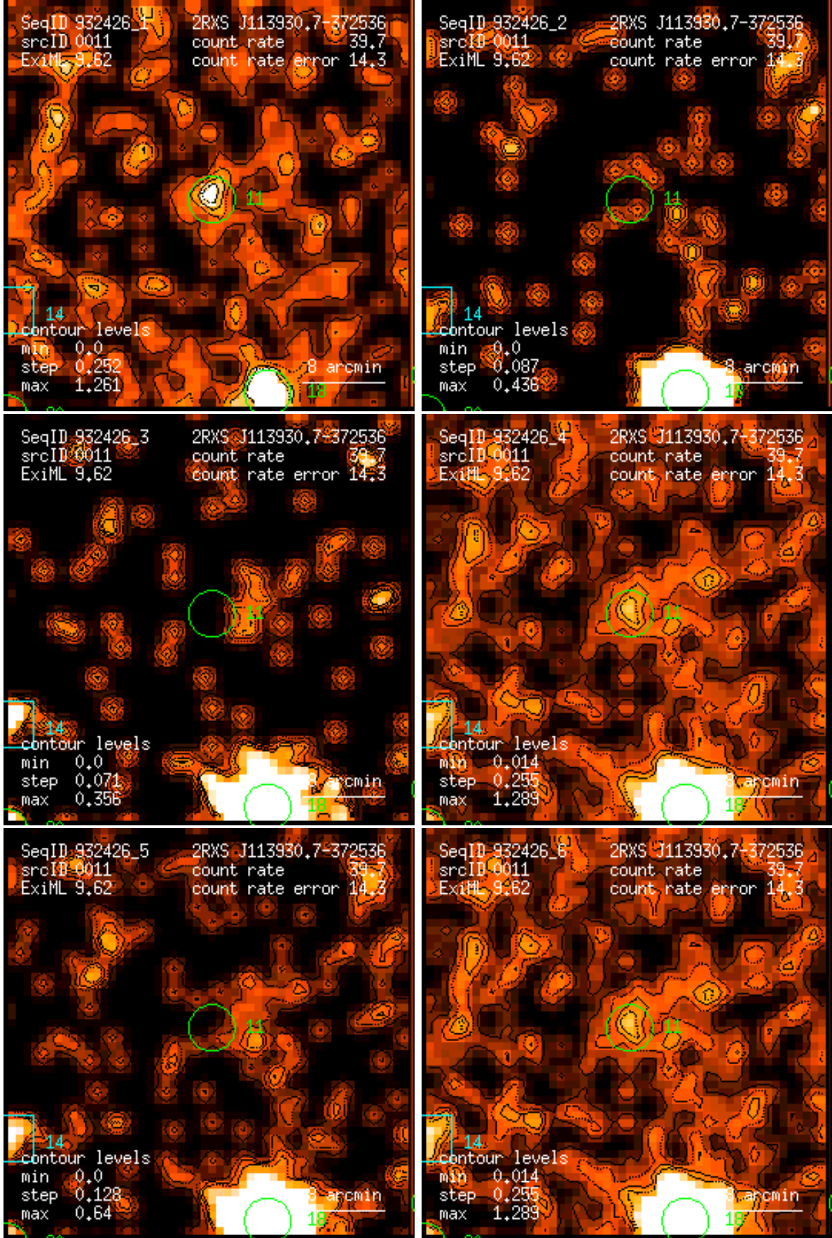
Figure 11: RASS 932426: detection 0011: band rate images, Gaussian filter: (1) PSPC channels 11 – 41, (2) 52 – 90, (3) 91 – 201, (4) 11 – 235, (5) 52 – 201, (6) 11 – 201. Broad band rates in counts/ks. Band rate contour levels in counts/ks/arcmin 2 .
