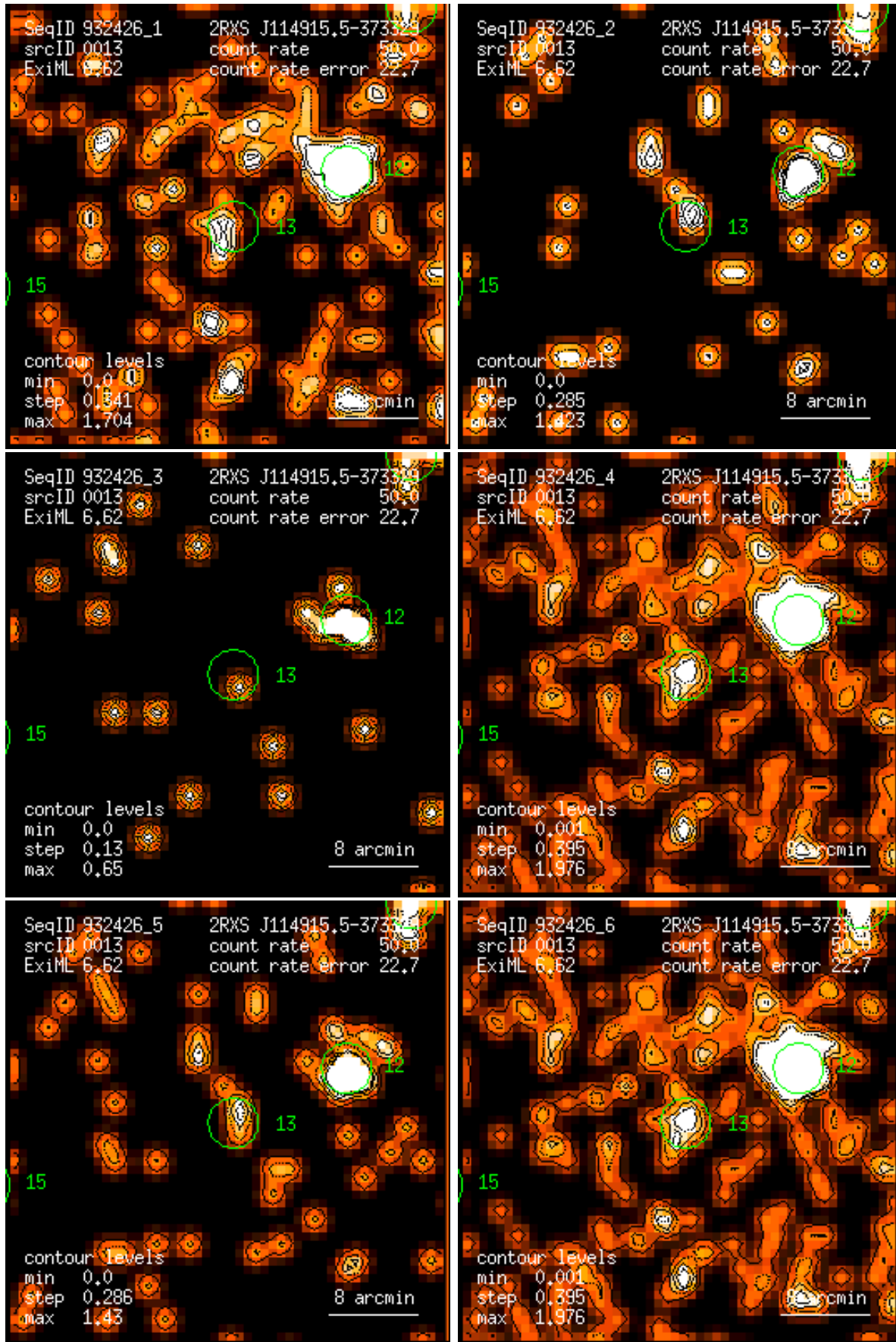
Figure 13: RASS 932426: detection 0013: band rate images, Gaussian filter: (1) PSPC channels 11 – 41, (2) 52 – 90, (3) 91 – 201, (4) 11 – 235, (5) 52 – 201, (6) 11 – 201. Broad band rates in counts/ks. Band rate contour levels in counts/ks/arcmin 2 .
