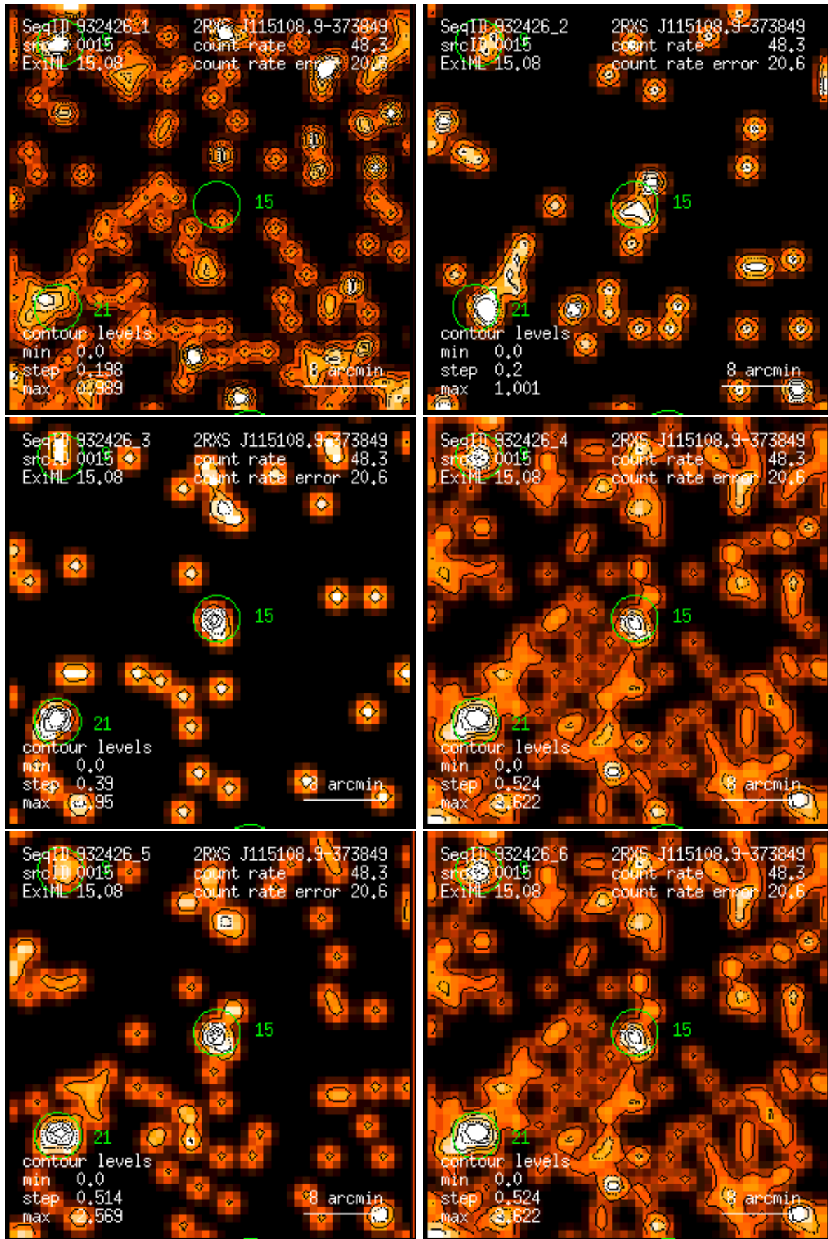
Figure 15: RASS 932426: detection 0015: band rate images, Gaussian filter: (1) PSPC channels 11 – 41, (2) 52 – 90, (3) 91 – 201, (4) 11 – 235, (5) 52 – 201, (6) 11 – 201. Broad band rates in counts/ks. Band rate contour levels in counts/ks/arcmin 2 .
