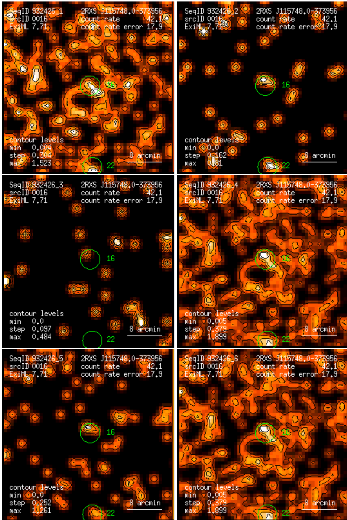
Figure 16: RASS 932426: detection 0016: band rate images, Gaussian filter: (1) PSPC channels 11 – 41, (2) 52 – 90, (3) 91 – 201, (4) 11 – 235, (5) 52 – 201, (6) 11 – 201. Broad band rates in counts/ks. Band rate contour levels in counts/ks/arcmin 2 .
