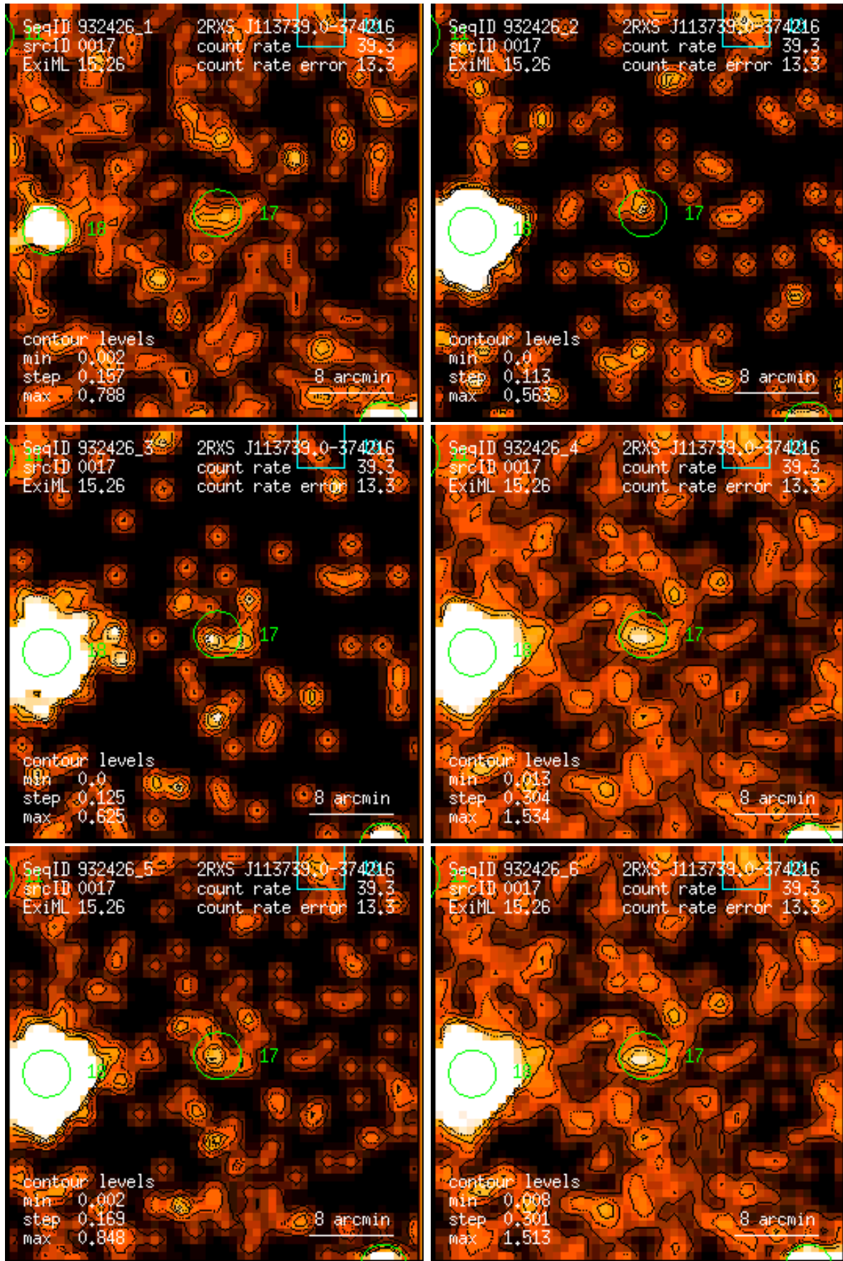
Figure 17: RASS 932426: detection 0017: band rate images, Gaussian filter: (1) PSPC channels 11 – 41, (2) 52 – 90, (3) 91 – 201, (4) 11 – 235, (5) 52 – 201, (6) 11 – 201. Broad band rates in counts/ks. Band rate contour levels in counts/ks/arcmin 2 .
