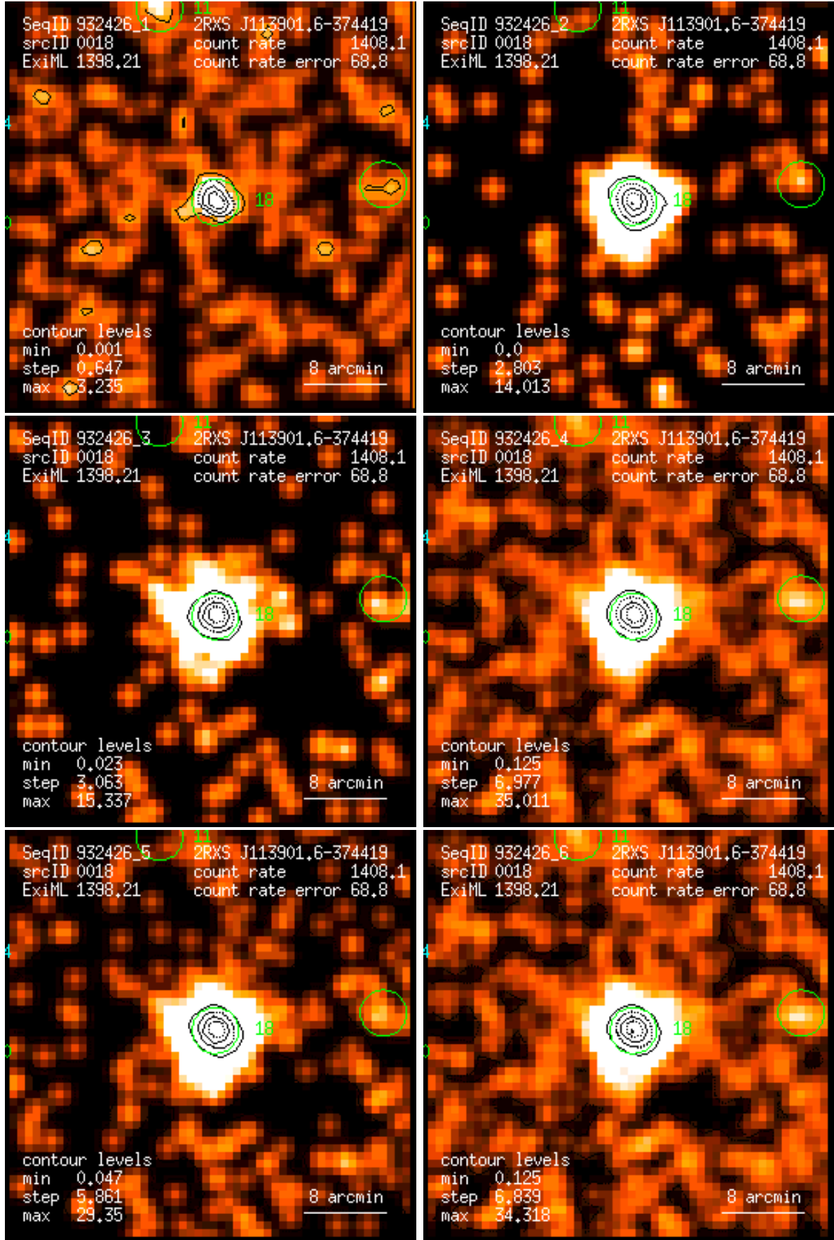
Figure 18: RASS 932426: detection 0018: band rate images, Gaussian filter: (1) PSPC channels 11 – 41, (2) 52 – 90, (3) 91 – 201, (4) 11 – 235, (5) 52 – 201, (6) 11 – 201. Broad band rates in counts/ks. Band rate contour levels in counts/ks/arcmin 2 .
