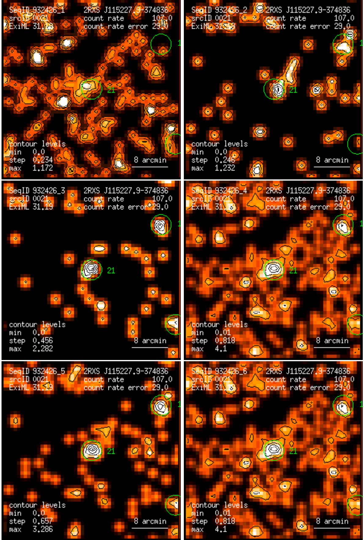
Figure 21: RASS 932426: detection 0021: band rate images, Gaussian filter: (1) PSPC channels 11 – 41, (2) 52 – 90, (3) 91 – 201, (4) 11 – 235, (5) 52 – 201, (6) 11 – 201. Broad band rates in counts/ks. Band rate contour levels in counts/ks/arcmin 2 .
