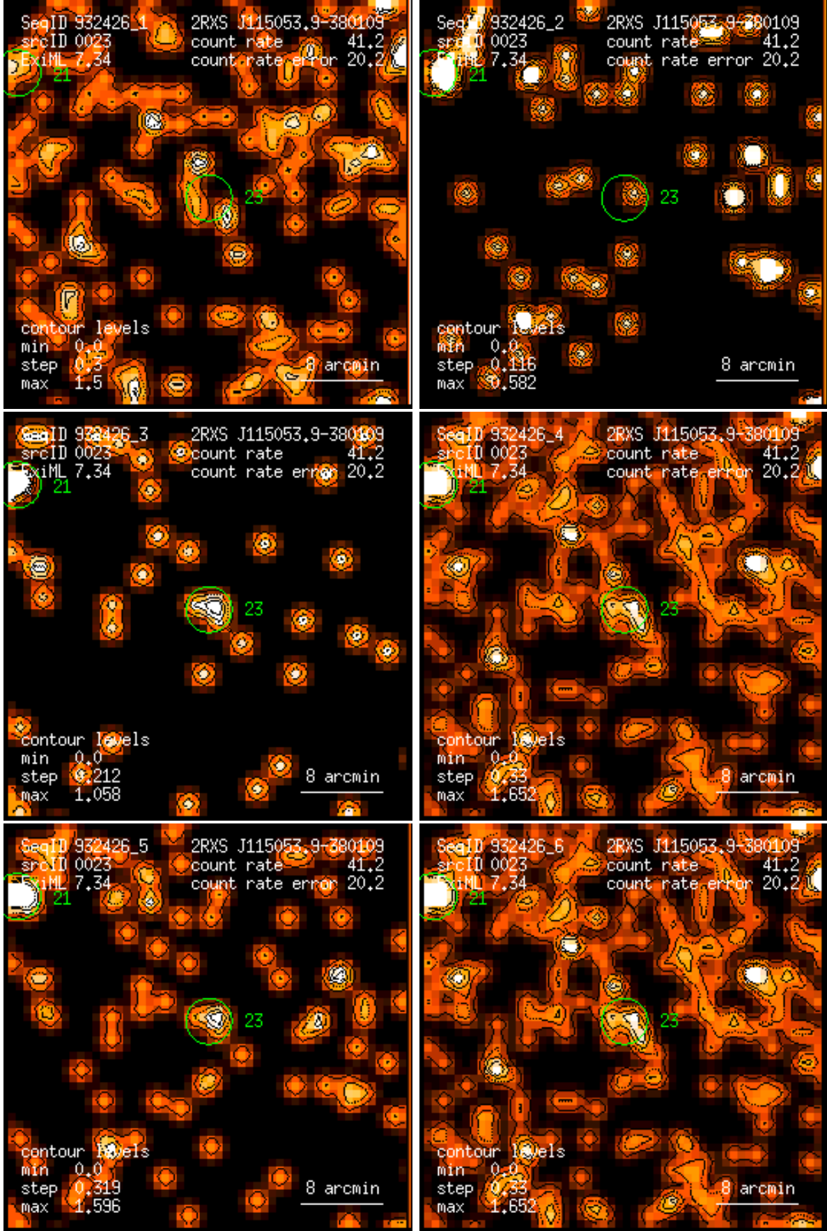
Figure 23: RASS 932426: detection 0023: band rate images, Gaussian filter: (1) PSPC channels 11 – 41, (2) 52 – 90, (3) 91 – 201, (4) 11 – 235, (5) 52 – 201, (6) 11 – 201. Broad band rates in counts/ks. Band rate contour levels in counts/ks/arcmin 2 .
