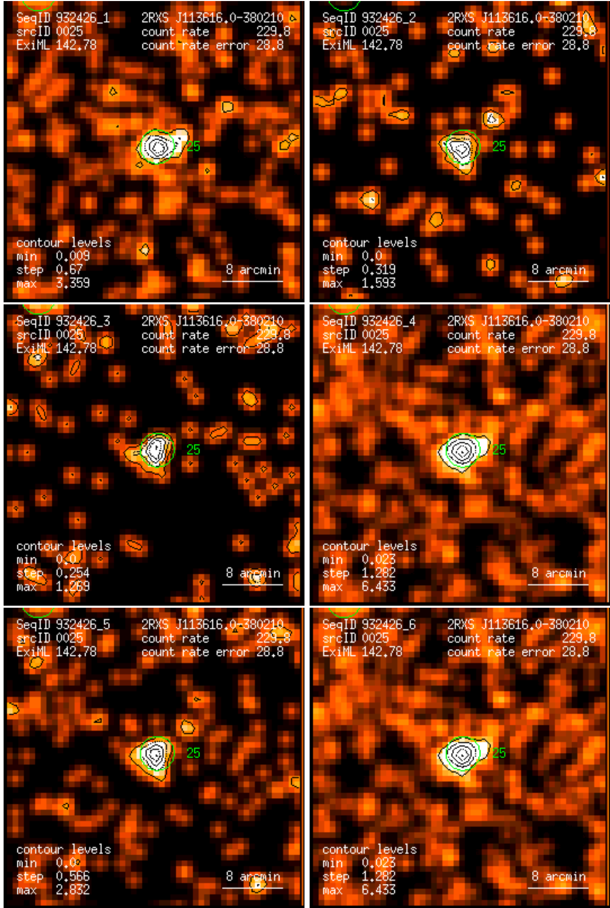
Figure 25: RASS 932426: detection 0025: band rate images, Gaussian filter: (1) PSPC channels 11 – 41, (2) 52 – 90, (3) 91 – 201, (4) 11 – 235, (5) 52 – 201, (6) 11 – 201. Broad band rates in counts/ks. Band rate contour levels in counts/ks/arcmin 2 .
