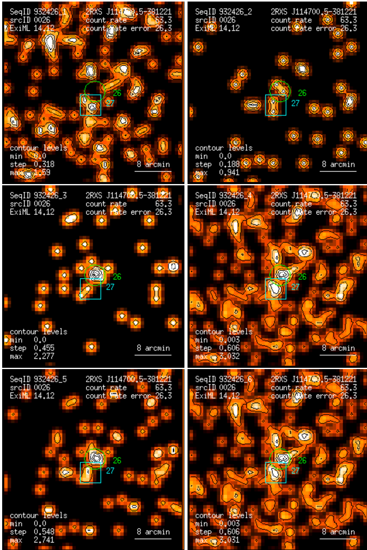
Figure 26: RASS 932426: detection 0026: band rate images, Gaussian filter: (1) PSPC channels 11 – 41, (2) 52 – 90, (3) 91 – 201, (4) 11 – 235, (5) 52 – 201, (6) 11 – 201. Broad band rates in counts/ks. Band rate contour levels in counts/ks/arcmin 2 .
