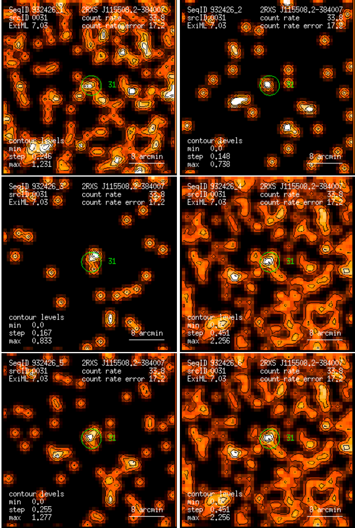
Figure 31: RASS 932426: detection 0031: band rate images, Gaussian filter: (1) PSPC channels 11 – 41, (2) 52 – 90, (3) 91 – 201, (4) 11 – 235, (5) 52 – 201, (6) 11 – 201. Broad band rates in counts/ks. Band rate contour levels in counts/ks/arcmin 2 .
