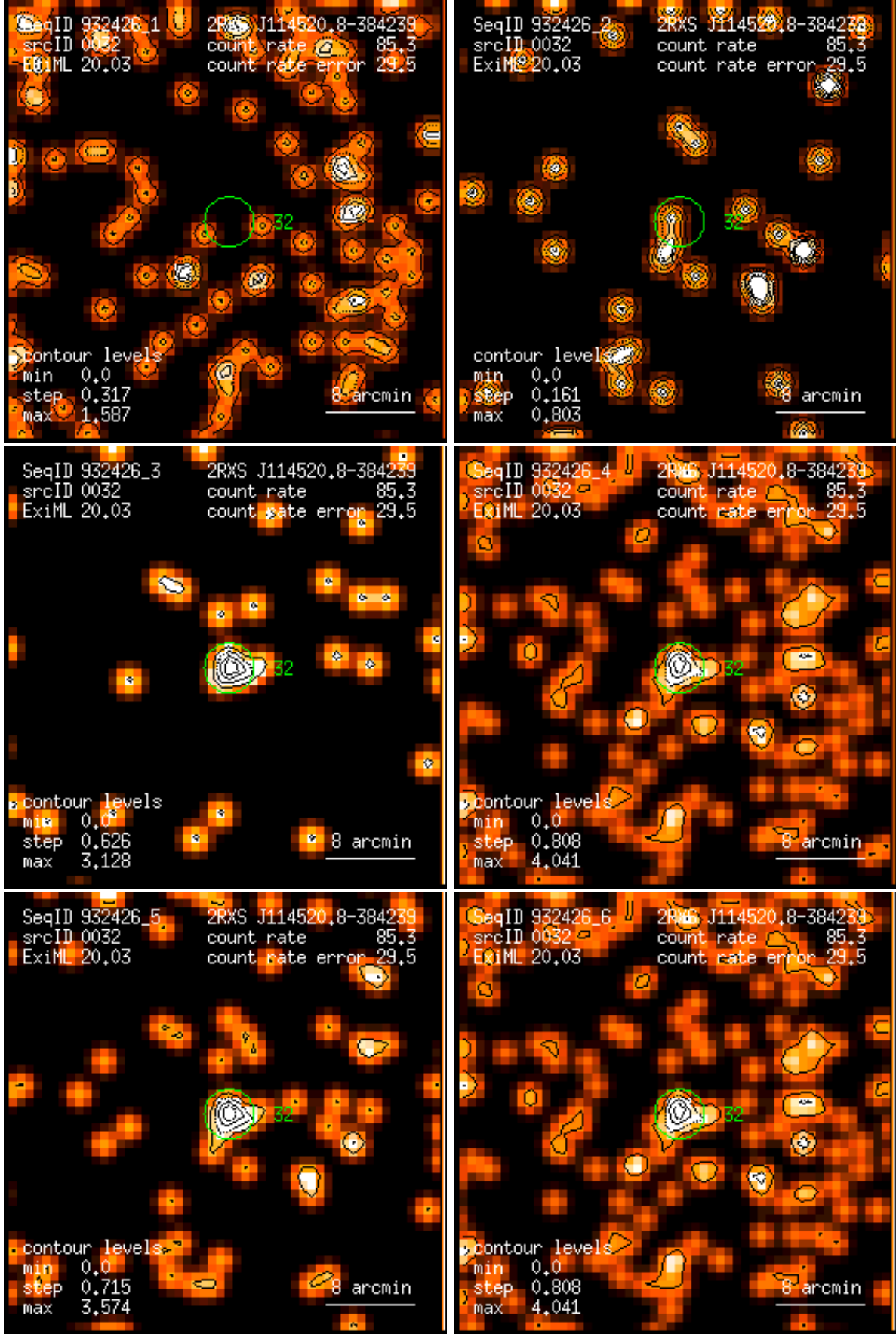
Figure 32: RASS 932426: detection 0032: band rate images, Gaussian filter: (1) PSPC channels 11 – 41, (2) 52 – 90, (3) 91 – 201, (4) 11 – 235, (5) 52 – 201, (6) 11 – 201. Broad band rates in counts/ks. Band rate contour levels in counts/ks/arcmin 2 .
